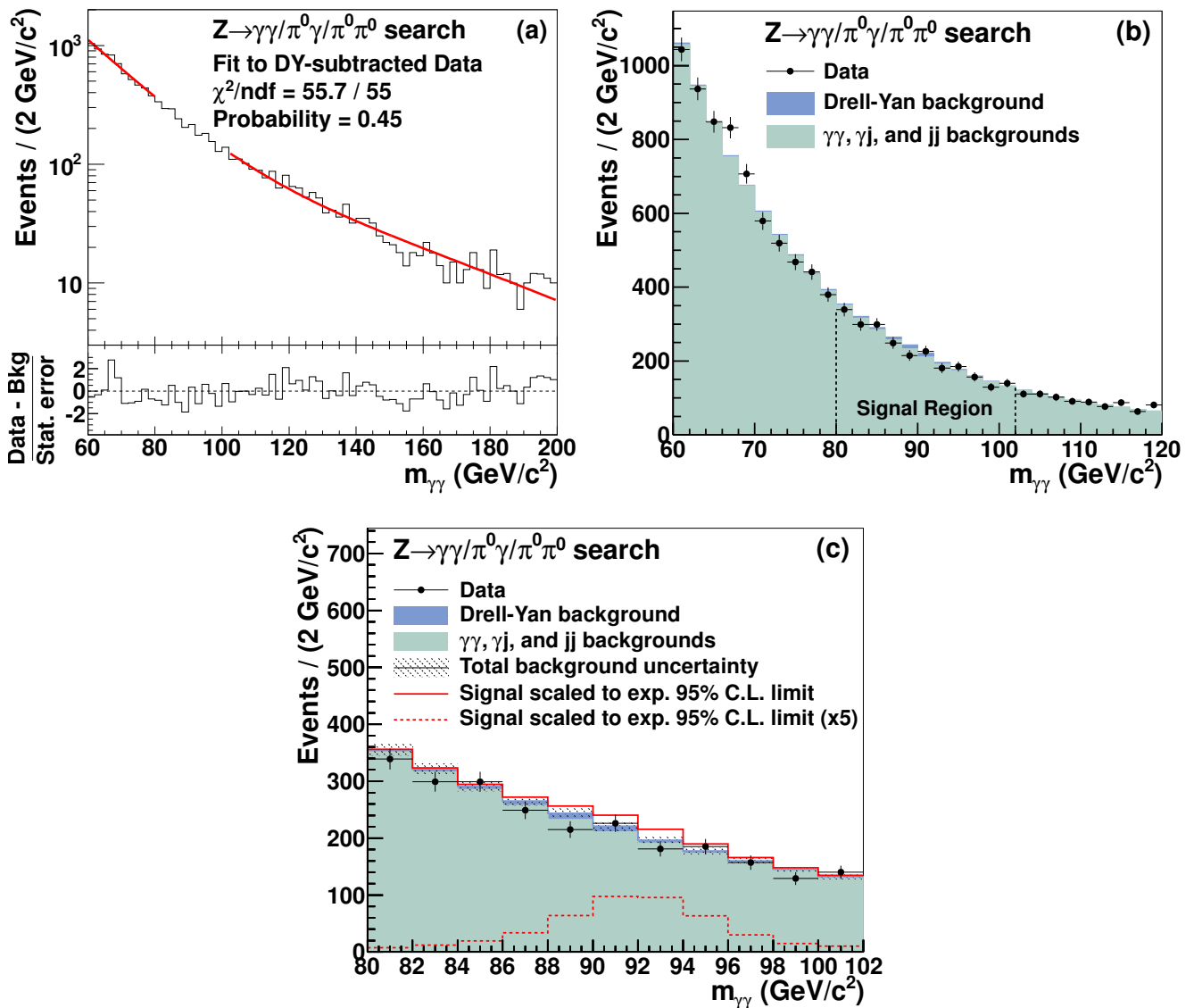
FIG. 2. (a) The diphoton mass distribution of the DY-subtracted data with the fit results overlaid. The gap in the fit function represents the excluded signal region. The lower subfigure shows the difference between the data and background predictions for the full 60–200 \text{GeV}/c^2 region, divided by the statistical uncertainty from the background prediction. (b) The diphoton mass distribution of the Drell-Yan and nonresonant ( \gamma\gamma , \gamma j , and jj ) backgrounds, compared to the data in the region 60–120 \text{GeV}/c^2 , which includes part of the fit region along with the 80–102 \text{GeV}/c^2 signal region. (c) The same distributions as (b), but for the signal region alone. Overlaid on the background is the predicted signal shape (solid line), scaled to the expected 95% C.L. upper limit. For better visibility, the same signal shape is also shown along the horizontal axis multiplied by 5 (dashed line).
