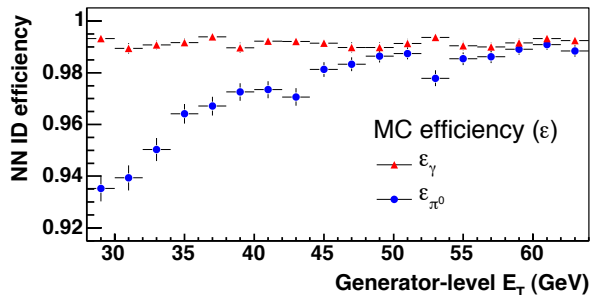
FIG. 1. Comparison of the \gamma and \pi^0 NN selection efficiencies, obtained using the special-purpose MC event generator. The efficiency is shown as a function of the generator-level E_T .
