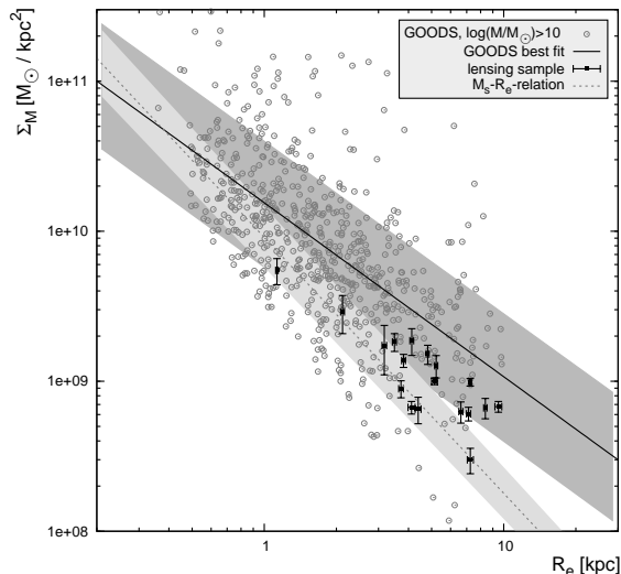
FIG. 2.— Stellar Surface Mass density versus effective radius. Early-type galaxies with stellar mass above 10^{10} M_\odot (open circles) selected from the Hubble Space Telescope/Advanced Camera for Surveys images of the Great Observatories Origins Deep Survey (GOODS) are shown together with our lensing sample (filled squares). The dashed line denotes the stellar mass to size relation from SDSS which accounts for early-type galaxies at z \sim 0.1 (Shen et al. 2003).
