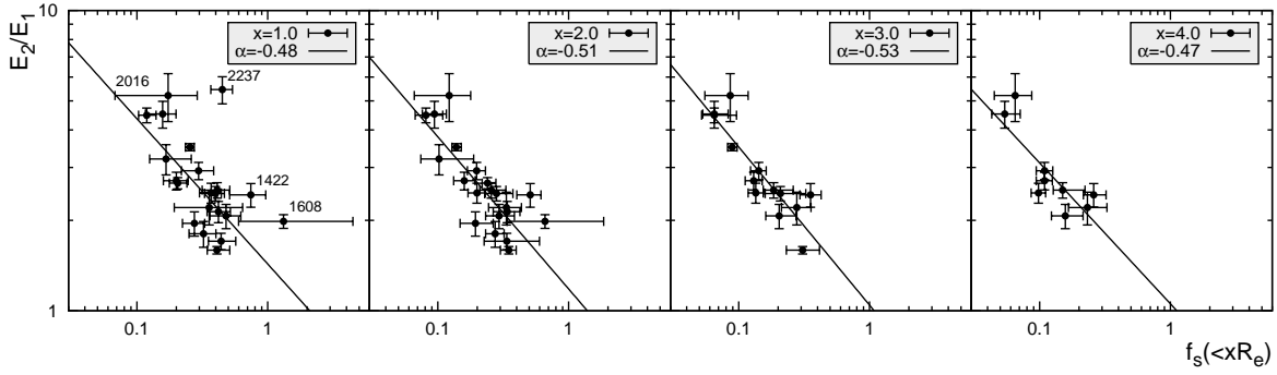
FIG. 13.— The stellar-mass fraction determined at 1.0, 2.0, 3.0 and 4.0 R_e versus E_2/E_1 . The solid line denotes the best fit of a power-law with slope \alpha . The fits exclude Q2237 and MG2016.
