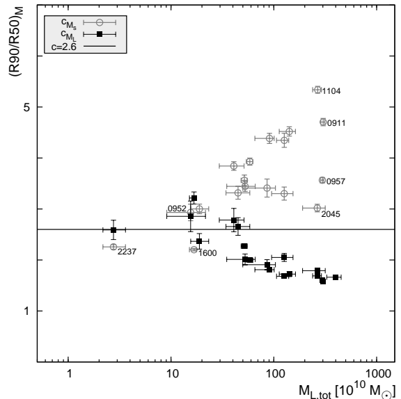
FIG. 12.— As in Fig. 11 but plotted against the total mass M_{L,tot} enclosed in 2R_e . The y-axis error bars represent for c_{M_L} the standard errors for mean concentrations of 300 models. For c_{M_s} the error bars correspond to the uncertainties originating from a 10% error in the flux per pixel.
