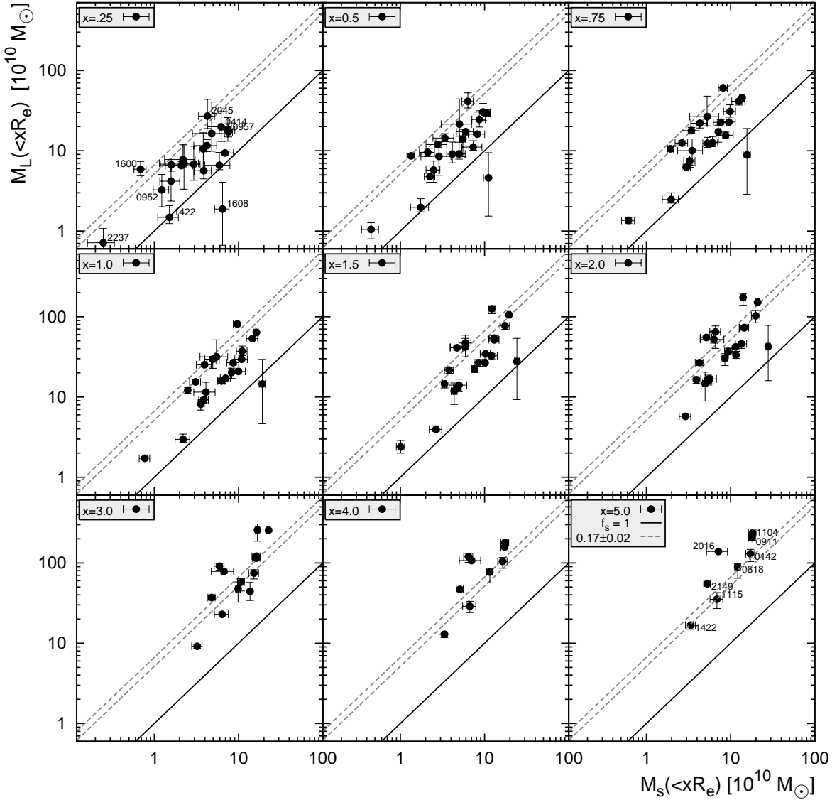
FIG. 6.— The panels show the enclosed M_L against enclosed M_s plane for a number of apertures, defined by the radial distance xR_e to the centre of the lensing galaxy, labelled by ‘ x ’ in the top-left corner of each panel. We cover a radial distance from 0.25 \times R_e to 5 \times R_e from upper left to lower right panels in conveniently chosen steps. The solid line denotes the equality of total and stellar mass, whereas the dashed lines represent the upper and lower limit of the global baryon fraction (Hinshaw et al. 2009).
