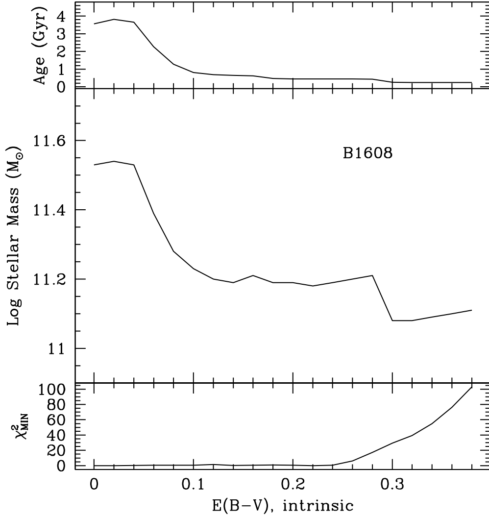
FIG. 16.— From top to bottom: Age, stellar mass and minimum \chi^2 versus reddening for the lens B1608.
