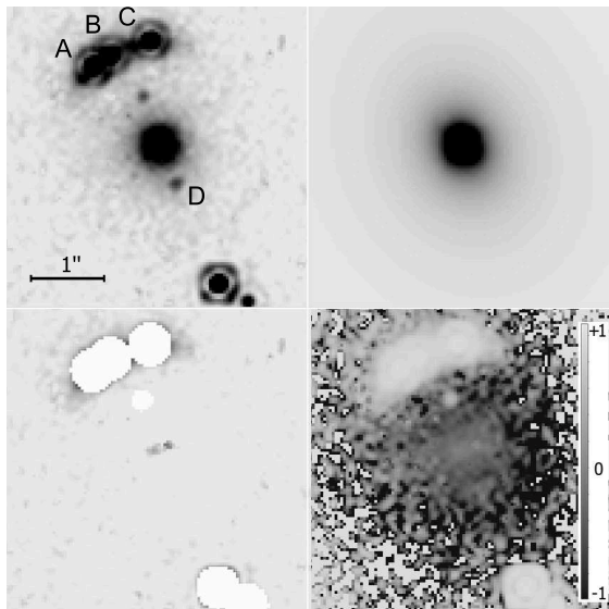
FIG. 1.— Upper left panel: original H-band NICMOS image of the lens system B2045. North is left and East is down. Best fits for the lensing galaxy could be obtained by masking out images A, B, C, the stellar objects south of the lens and a “blob” West of the lensing galaxy. Upper right panel: model for the lensing galaxy. Lower left panel: Residual image. Lower right panel: Residual divided by original image.
