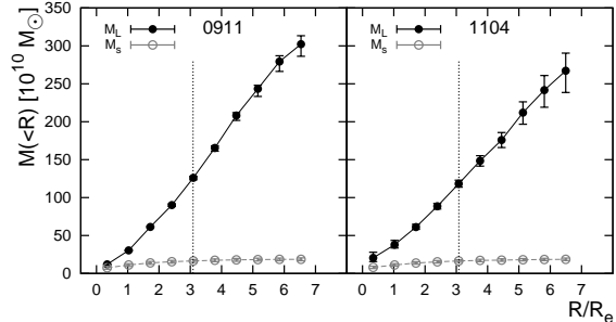
FIG. 5.— As in Fig. 3 for the high mass lenses RXJ0911 and HE1104.
