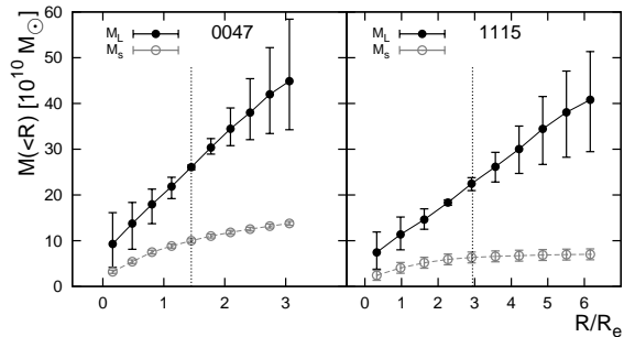
FIG. 3.— Cumulative stellar mass and total lensing mass content against radius in terms of R_e for the low mass lenses Q0047 and PG1115. The thin dotted vertical line marks the outermost image position R_{\text{lens}} .
