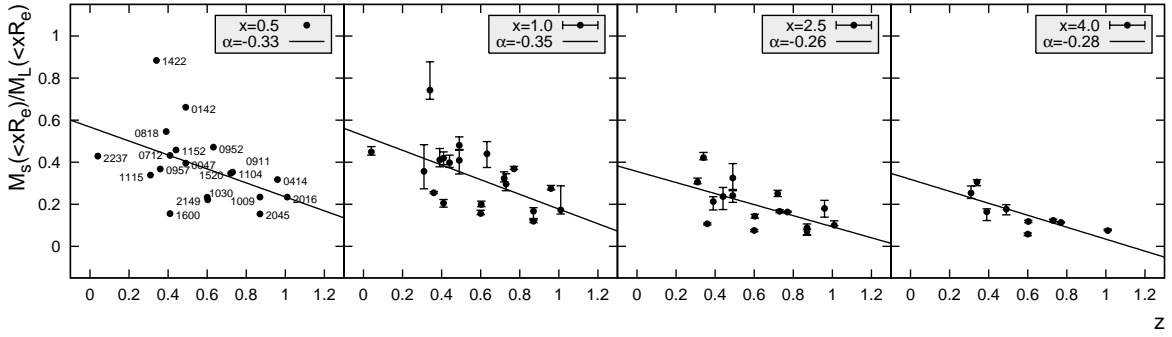
FIG. 10.— The stellar-mass fraction determined at 0.5, 1.0, 2.0 and 4.0 R_e against redshift.
