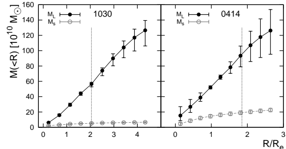
FIG. 4.— As in Fig. 3 for the intermediate mass lenses B1030 and MG0414.
