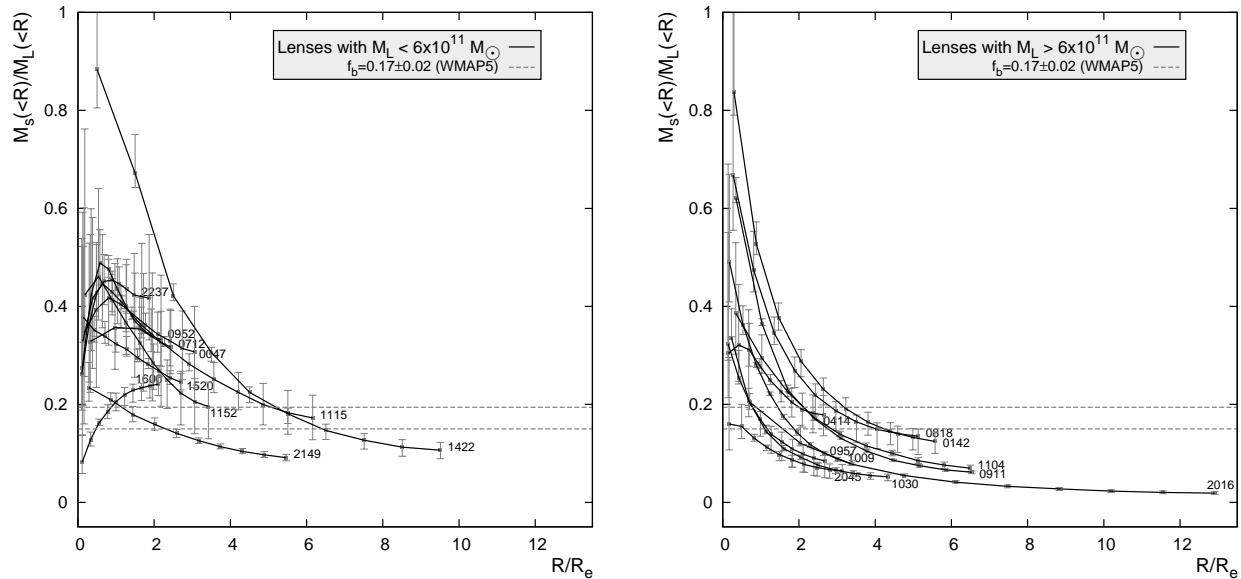
FIG. 7.— Left panel: Stellar-mass fraction against radius in effective radii for lenses with lensing mass below 6 \times 10^{11} M_{\odot} . Right panel: Similar, but for lenses with lensing mass above 6 \times 10^{11} M_{\odot} .
