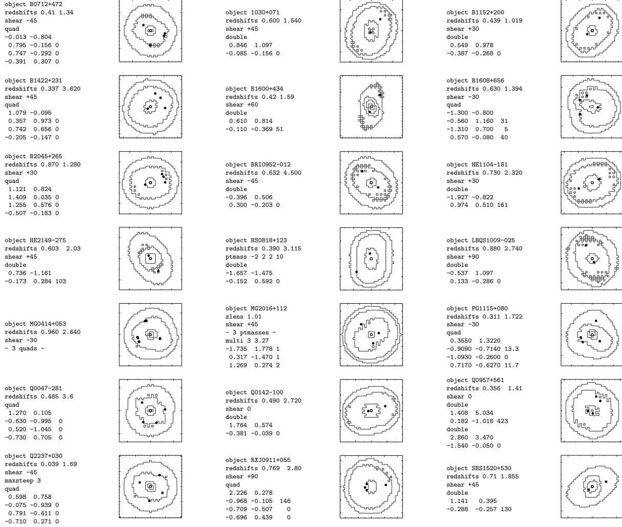
FIG. 15.— PIXELENS input data and projected mass distribution for the lensing sample. The black dots mark the multiple images. All maps have a radius of 15 pixel. All mass maps have a radius of 2 R_{\text{lens}} , which corresponds roughly to 2 R_{E_{\text{in}}} . All lens properties as well as respective length specifications are in Table 1.
