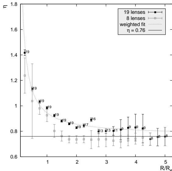
FIG. 8.— Slope of the M_s -to- M_L relation taken from Fig. 6 plotted against the distance to the centre in terms of effective radii. The median slopes are determined via a bootstrapping fitting method with 10^4 realizations to compute meaningful standard errors for a sample of 19 lenses (filled squares) and a reduced 8 lens sample (open squares). The numbers at the filled squares give the number of lenses probed out to the respective radius. The dotted line represents a weighted best fit of \eta(R) \sim 1/R + \text{const.}
