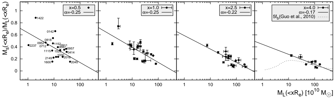
FIG. 9.— The stellar-mass fraction determined at 0.5, 1.0, 2.5 and 4.0 R_e against total mass. The best fits are found for the sample excluding lenses with mean stellar-mass fractions above 1 at R_e , which is the case only for B1608.
