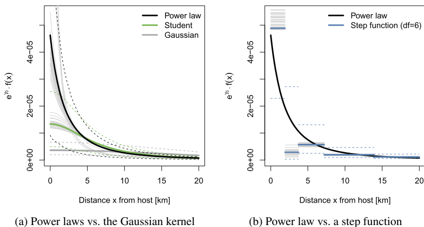
FIG. 3. Estimated spatial interaction functions—appropriately scaled by the epidemic intercept \exp(\gamma_0) . The dashed lines represent 95% confidence intervals obtained as the pointwise 2.5% and 97.5% quantiles of the functions evaluated for 999 samples from the asymptotic multivariate normal distribution of the affected parameters. The light grey lines are estimates obtained from a sensitivity analysis with repeated random tie-breaking.
