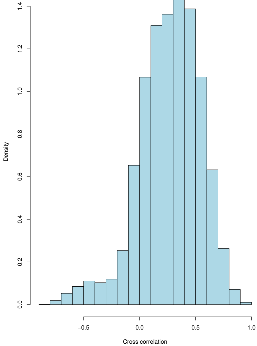
Figure 2: Histogram of the 208 \cdot 209/2 = 21,736 cross correlations between the excess returns of the 209 hedge funds. Since it is not true that the majority of these correlations are close to zero, the weak dependence assumption of Storey et al. (2004) is clearly violated.
