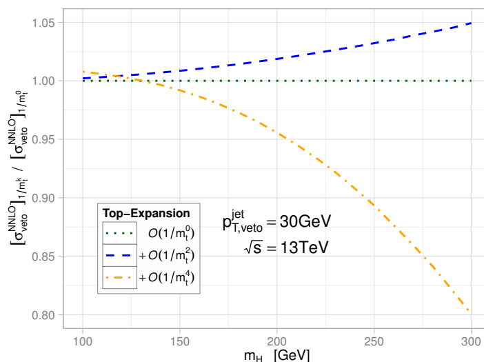
Figure 9. Higgs+0-jet cross section at NNLO including terms up to 1/m_t^k as a function of m_H normalized to heavy-top limit ( k = 0 ) for p_{T,veto}^{\text{jet}} = 30 \text{ GeV} . Dotted/dashed/dash-dotted: k = 0/2/4 .
