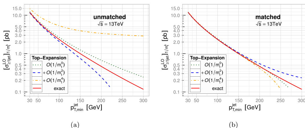
Figure 6. Inclusive Higgs+jet cross section at LO including terms up to 1/m_t^k as a function of p_{T,\min}^{\text{jet}} . Dotted/dashed/dash-dotted: k = 0/2/4 . (a) unmatched; (b) matched according to eq. (3.5).
