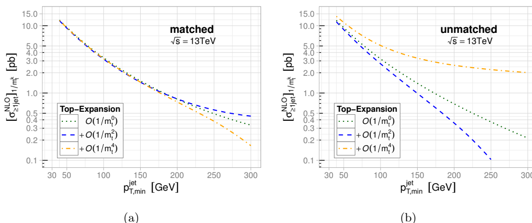
Figure 10. Inclusive Higgs+jet cross section at NLO including terms up to 1/m_t^k as a function of p_{T,\text{min}}^{\text{jet}} . Dotted/dashed/dash-dotted: k = 0/2/4 . (a) matched according to eq. (3.6); (b) unmatched.
