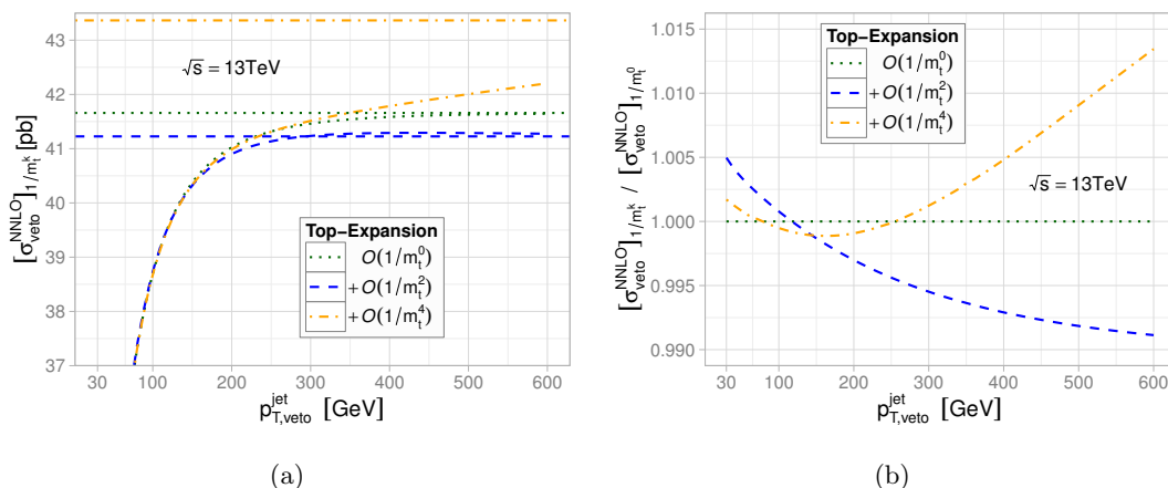
Figure 8. Higgs+0-jet cross section at NNLO including terms up to 1/m_t^k as a function of p_{T,\text{veto}}^{\text{jet}} . Dotted/dashed/dash-dotted: k = 0/2/4 . (a) absolute; for reference, the horizontal lines display the corresponding total cross sections in the three approximations; (b) normalized to k = 0 .
