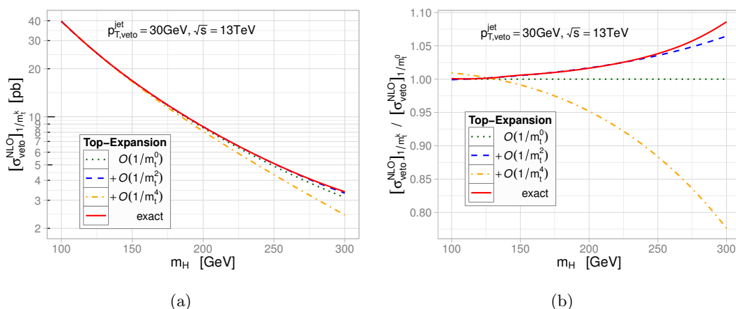
Figure 4. Higgs+0-jet cross section at NLO including terms up to 1/m_t^k as a function of m_H for p_{T,\text{veto}}^{\text{jet}} = 30 GeV. Dotted/dashed/dash-dotted: k = 0/2/4 . (a) absolute; (b) normalized to k = 0 .
