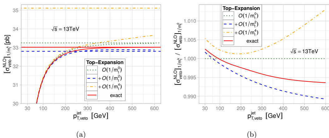
Figure 5. Higgs+0-jet cross section at NLO including terms up to 1/m_t^k as a function of p_{T,veto}^{\text{jet}} . Dotted/dashed/dash-dotted: k = 0/2/4 . (a) absolute; (b) normalized to k = 0 .
