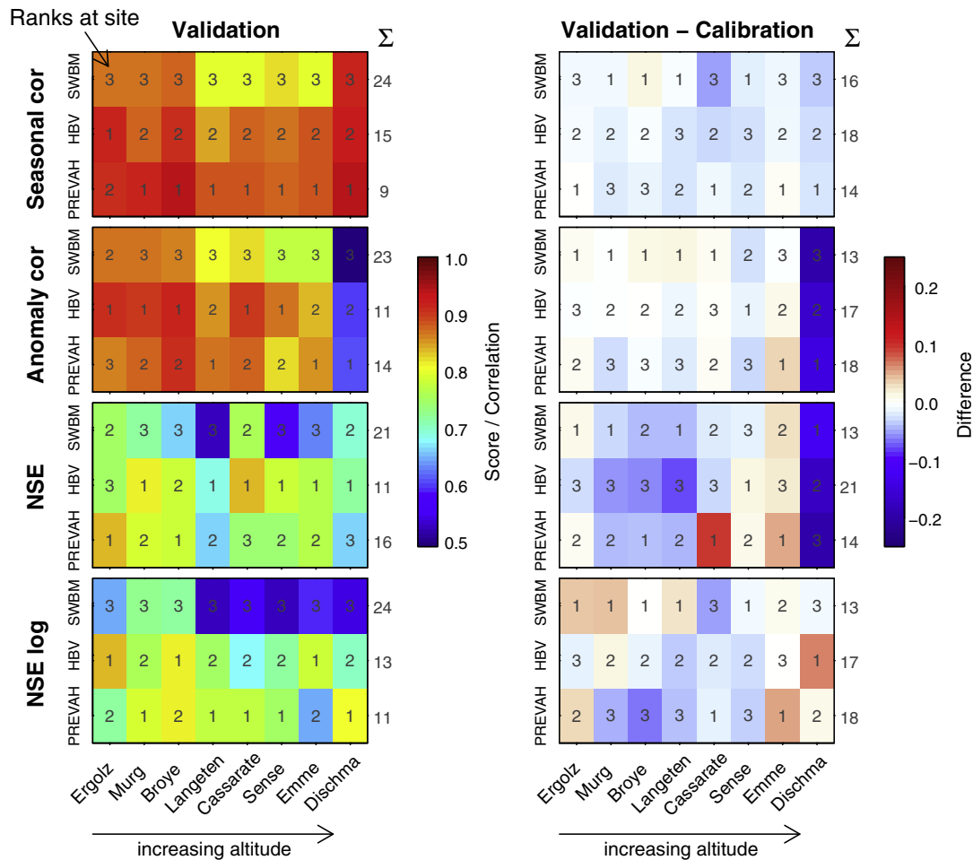
Fig. 4. Agreement between modeled and observed runoff, expressed as seasonal correlation, anomaly correlation and Nash–Sutcliffe efficiency. The results for the validation period 1997–2009 are displayed on the left side, the respective difference with results from the calibration period 1987–1996 is shown on the right side (validation minus calibration results). For each site and quantity ranks of the models are displayed, with the sum over all sites on the right side.
