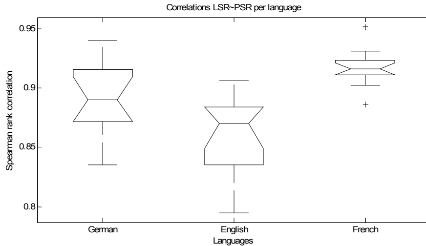
Figure 2: Box plot showing the distribution of Spearman rank correlation coefficients for the correlation between psr and lsr.
