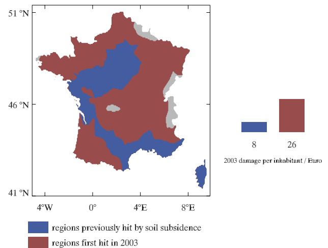
Fig. 7. Drought regions in France. Blue: Regions where simulated soil water deficits exceed 200 mm at least half of the years during the reference period (1961–1990), as well as in 2003. Red: Regions also affected in 2003, but not regularly during the reference period. Gray: Unaffected regions. The numbers on the right hand side represent estimated observed 2003 damage per capita for the blue and red regions.
