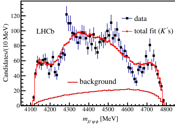
FIG. 1. Distribution of m_{J/\psi\phi} for the data and the fit results with a model containing only K^{*+} \rightarrow \phi K^+ contributions.
