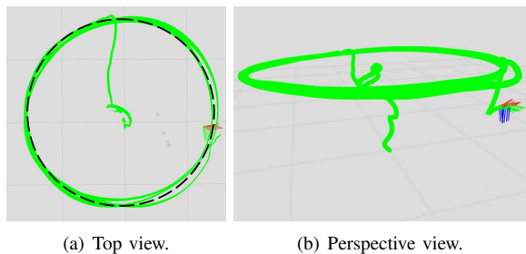
Fig. 7. Experiment 2: Fast circles in a low-lit room. The trajectory estimated by our pipeline is the green line. The commanded trajectory is the superimposed black dashed line.
