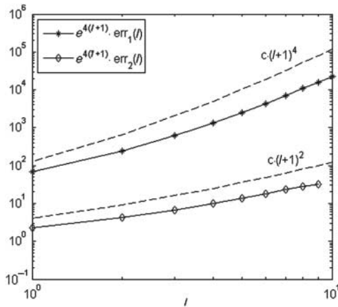
FIG. 6. Log-log scale plot of e^{4(l+1)} \cdot err_j(l) for j = 1, 2 .
