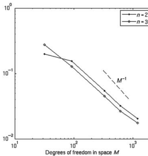
FIG. 10. Relative error err_{rel} for T = 2 , g(x, t) = \sin(t)^4 e^{-0.5t} Y_n^0 with n = 2, 3 and piecewise constant approximation in space.
