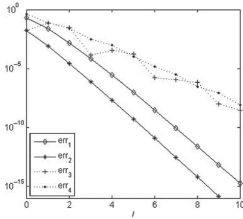
FIG. 5. err_j(l) for j = 1, 2, 3, 4 .
