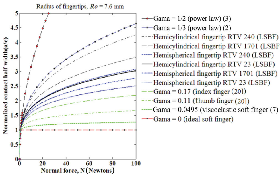
Fig. 7. (Colour online) The normalized half width contact as a function of the normal force (\frac{a_{cy}}{c_{cy}}) = N^{\gamma_{cy}} .
