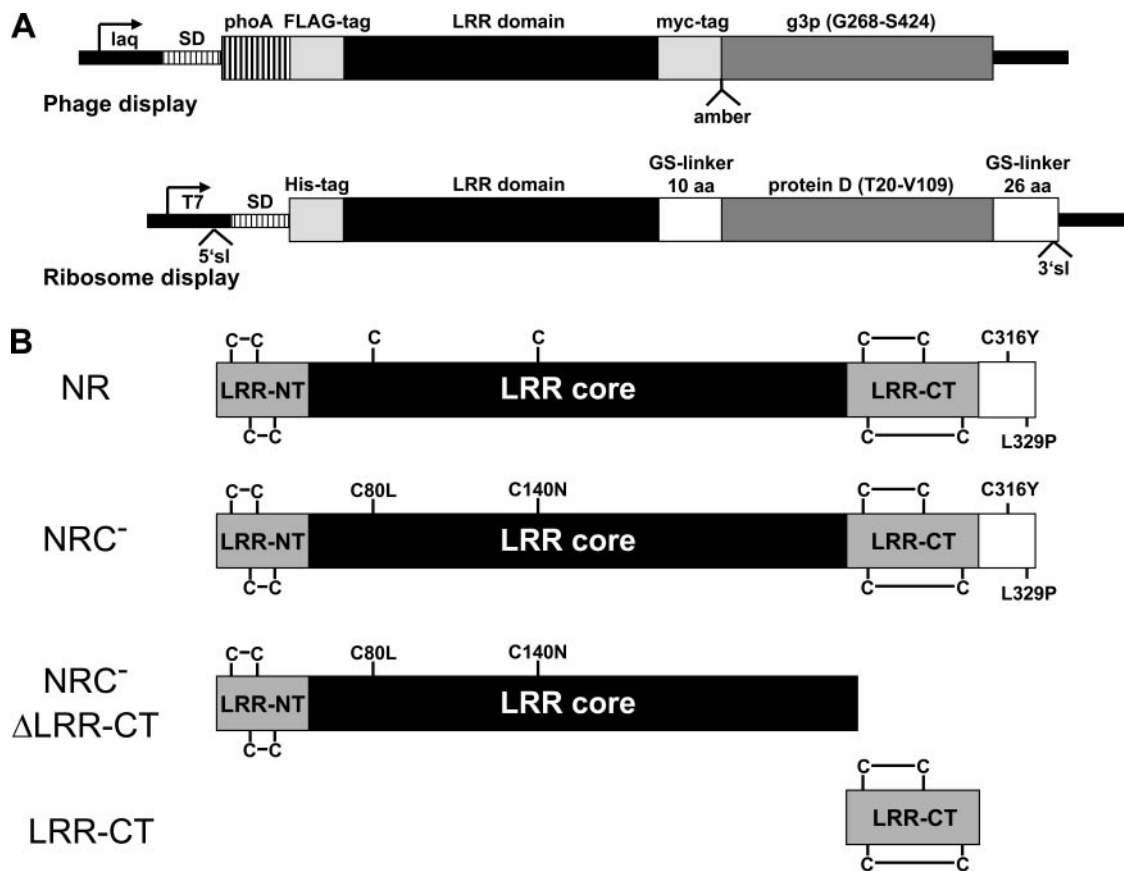
Fig. 2. (A) Schematic representation of the fusion constructs used for phage display (upper graph) and ribosome display (lower graph). (B) Schematic representation of variants of the Nogoceptor ligand binding domain (residues 24–331) used in these studies. The conserved disulfide bridges in the N- and C-terminal ‘capping modules’ (LRR-NT, LRR-CT) and the free cysteines in the LRR core region are indicated. Both free cysteines are mutated to the respective consensus residues in variant NRC - . The LRR core region is composed of 8.5 LRR modules. The mutations in the far C-terminal overhang of 22 amino acids represent the changes of the macaque to the human receptor sequence.
