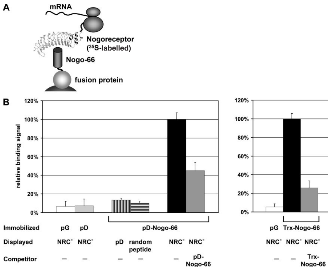
Fig. 3. RIA of ribosomal complexes displaying [ 35 S]methionine-labelled Nogoreceptor domains. (A) Schematic representation of the binding assay. (B) Binding of ribosomal complexes displaying in vitro translated and 35 S-labelled Nogoreceptor to Nogo-66 fusion proteins, immobilized on paramagnetic beads, was investigated. Immobilized refers to the protein coated on the magnetic beads, displayed to the protein translated and connected to the ribosomes and competitor to protein present in solution. As negative controls, the binding of Nogoreceptor-displaying ternary complexes to other proteins was investigated: binding to beads coated with protein G (white bars) or to beads coated with lambda phage protein D missing the C-terminal Nogo-66 insertion (light grey column). As further negative controls the non-specific binding of ribosomal complexes displaying unrelated proteins on immobilized pD-Nogo-66 was assessed: binding of ribosomal complexes only displaying protein D (vertically striped bars) or a protein derived from a random sequence library (horizontally striped lines). Black bars represent specific binding to Nogo-66, being immobilized either as a fusion to protein D or as a fusion to thioredoxin. Signals observed when the free ligand Nogo-66 is added as a competitor at a concentration of 4 μM (grey bars). All reactions were performed in the presence of 5 mg/ml BSA and 250 μg/ml S.cerevisiae RNA. Signals are normalized to the binding signal of the respective Nogo-66 fusion protein.
