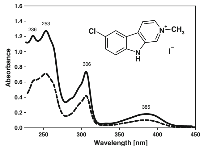
Fig. 2 Structure and absorption spectra of natural nostocarboline [in 60% (v/v) aqueous MeOH; dashed line] and synthetic nostocarboline iodide (in 100% MeOH; solid line)
