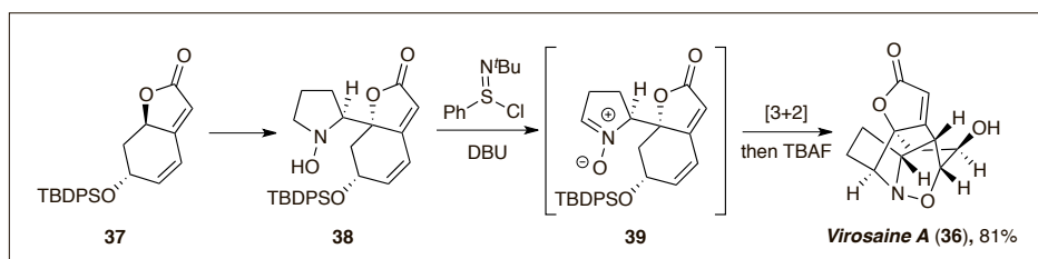
Scheme 7. Total synthesis of virosaine A via a proposed [3+2]-nitron olefin cycloaddition.
