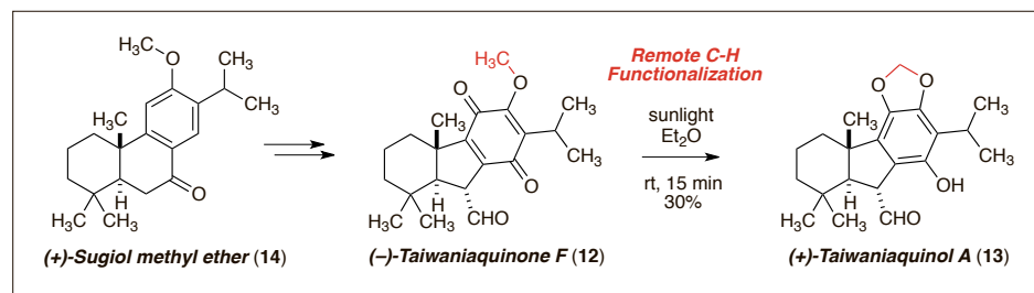
Scheme 3. Total synthesis of taiwaniaquinone F ( 12 ) and its biomimetic remote C–H functionalization to taiwaniaquinol A ( 13 ).
