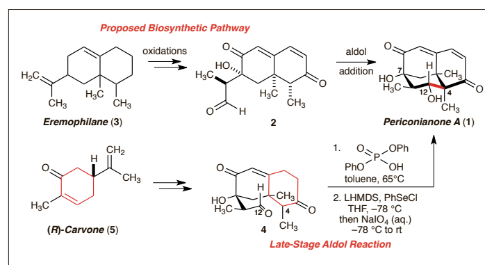
Scheme 1. Proposed biosynthetic pathway and synthetic strategy to periconianone A ( 1 ).
