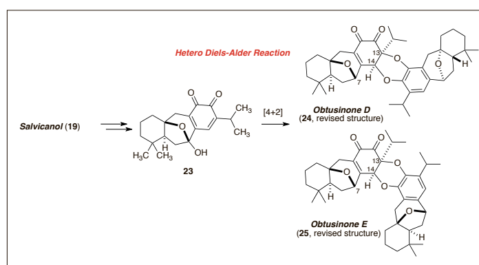
Scheme 5. Biomimetic dimerization of 23 in a hetero Diels-Alder reaction to the natural products obtusinone D ( 24 ) and E ( 25 ).
