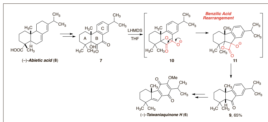
Scheme 2. Biomimetic total synthesis of taiwaniaquinone H ( 6 ) via a benzilic acid rearrangement.
