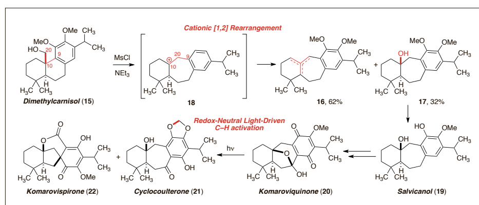
Scheme 4. Collective synthesis of the natural products salvicanol ( 19 ) and komaroviquinone ( 20 ) using a biosynthetically proposed cationic [1,2]-rearrangement, and redox-neutral light-driven C-H activation of 20 to cyclocoulerone ( 21 ) and komarovispirone ( 22 ).
