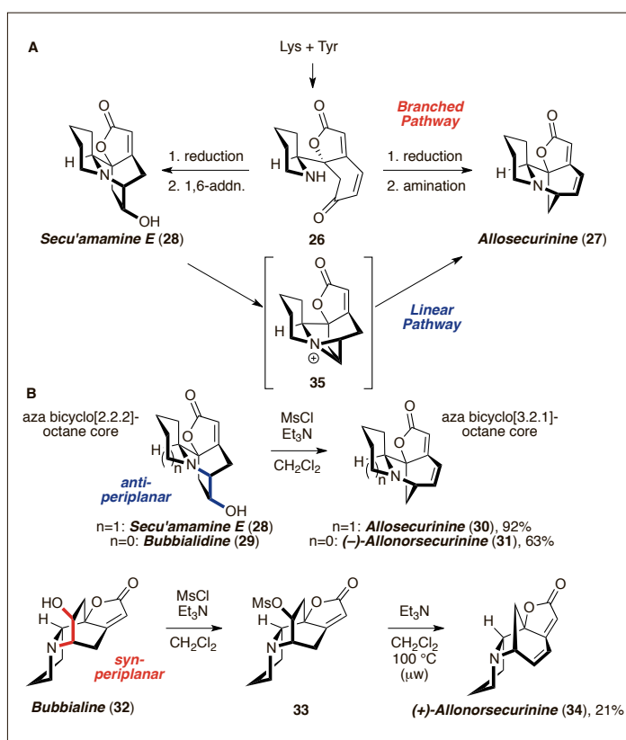
Scheme 6. A) Biogenetic hypothesis to Securinega alkaloids; B) Dehydrative rearrangement of Securinega alkaloids.
