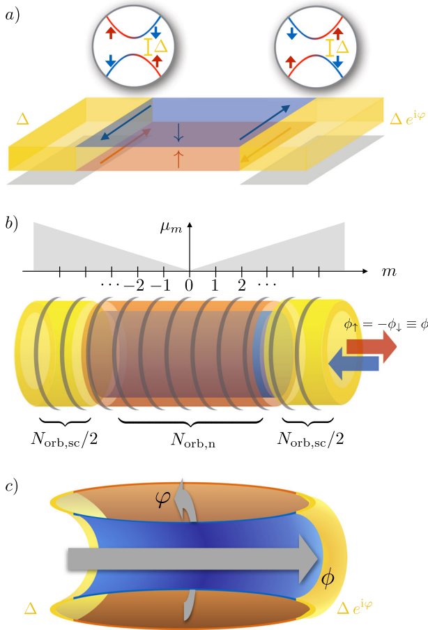
Fig. 1 Schematics of the physical geometry and the one used for the numerical investigation. a Fractional topological insulator heterostructure in which carriers with spin up and down (red and blue) form a fractional quantum Hall state with opposite chirality. Proximity to superconducting reservoirs (yellow) induces a superconducting gap in their edge channels. To study the Josephson effect, relative phase \phi between the left and right superconducting order parameter is included. b When imposing periodic boundary conditions along the edges, resulting in a cylinder geometry, each edge carries a topological degree of freedom. The boundary conditions can be twisted by inserting a flux \phi into the cylinder for spin up electrons and -\phi for spin down electrons. In the Landau gauge orbitals are localized along the cylinder, where we consider N_{\text{orb},n} and N_{\text{orb},sc} normal and superconducting orbitals, respectively. The typical separation between orbitals is \frac{2\pi\ell_B^2}{L_y} , where L_y is the cylinder perimeter. The droplet is confined by a linear potential \mu_m . c With the counter-propagating edges gapped out, the bilayer FQH state on the cylinder is topologically equivalent to a single layer FQH state on a torus, where the fluxes \phi and \varphi run through its two noncontractible cycles and can be used to explore its topological ground state degeneracy. It is thus topologically equivalent to the ground state degeneracy of the gapped edge modes
