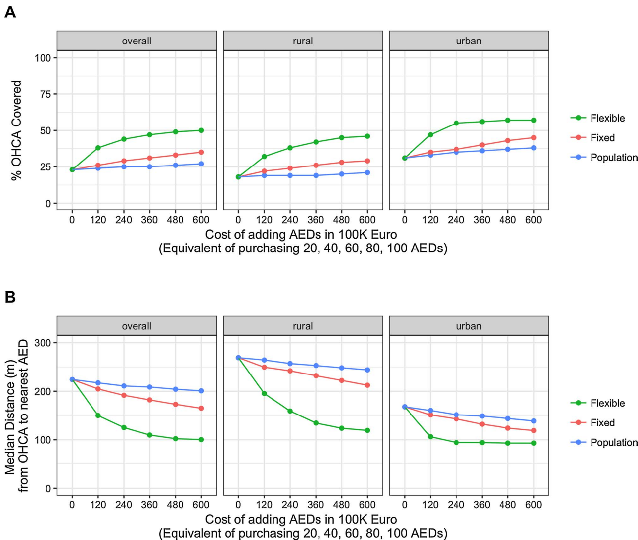
Fig. 1. Panel A shows OHCA test set coverage for flexible location, fixed location, and population models. Panel B shows the median distance from OHCA events to the nearest AED for flexible location, fixed location, and population models. All results use the test set coverage and distances, and are split by the overall area, and rural and urban areas.
