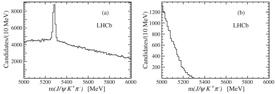
FIG. 3. For the P_{B^0}^+ \rightarrow J/\psi K^+ \pi^- p decay search (mode I ), the invariant mass of J/\psi K^+ \pi^- combinations in the (a) region above threshold and in the (b) signal region. The peak in the sideband region results from B^0 decays.
