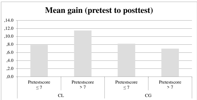
Figure 2. Mean gain in CL vs. CG condition by pretest computation competence
