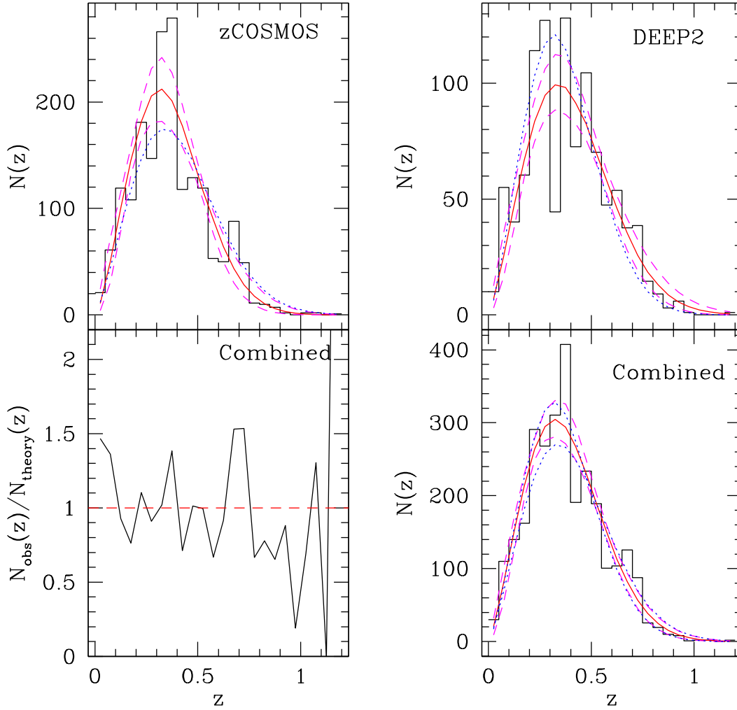
Figure 5. Top: Rescaled redshift histograms for the matches between the source catalog and the zCOSMOS (left) and DEEP2 (right) sample with best-fit histograms. The black histogram is the observed data, the smooth red curve is the best-fit histogram, the dashed magenta lines are the \pm 1\sigma errors, and the dotted blue line is the best-fit redshift histogram for the other survey. Bottom right: Same as above, for combined sample, with the dotted blue lines showing the results for each survey separately. Bottom left: ratio of observed to best-fit N(z) for the combined sample.
