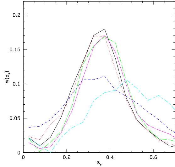
Figure 12. Smoothed weight as a function of source redshift for several lens redshifts in DEEP2 and zCOSMOS, to minimize the effects of LSS. This plot is a smoothed version of the lower right panel of Fig. 10, with the same line types and colours as in that plot. The smoothing algorithm is described in the text.
