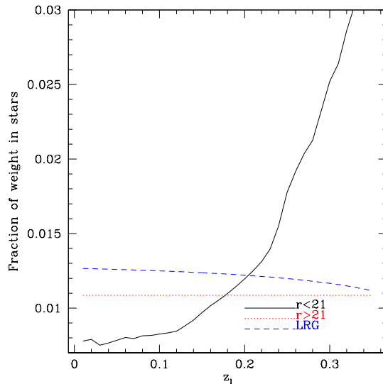
Figure 18. Fraction of the weight for our three source samples that is attributed to stellar contamination as a function of lens redshift.
