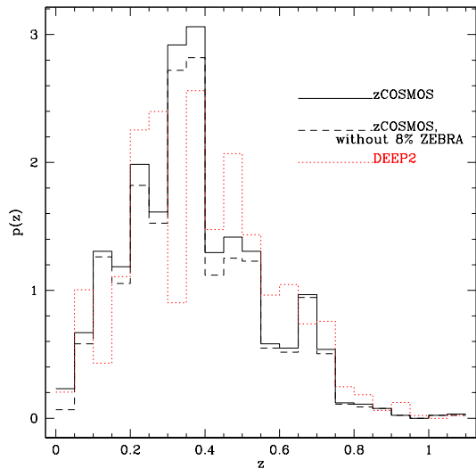
Figure 2. Redshift histogram for the matches between the source catalog and the spectroscopic samples.
