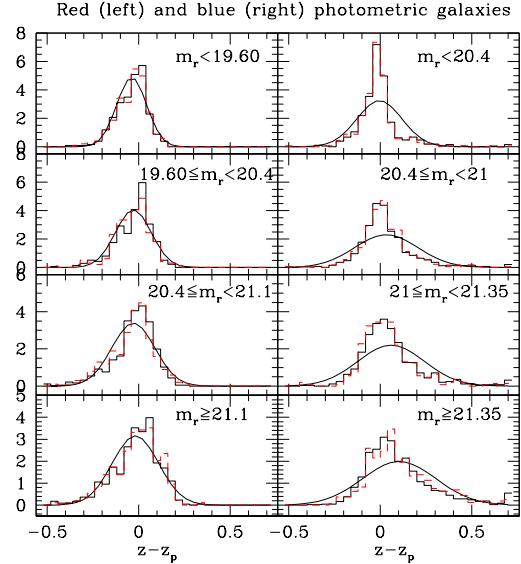
Figure 17. Photoz error distributions for the SDSS/ZEBRA method as a function of colour and magnitude for the full flux-limited sample (black, solid) and for the lensing sources (red, dashed). We have also shown the Gaussians with the mean and scatter from Table 10.
