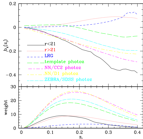
Figure 7. Redshift bias b_z(z_l) (top) and weight (bottom, arbitrary units) for many methods of source redshift determination as described in the text. Errorbars are not shown, to make the plot simpler to read.
