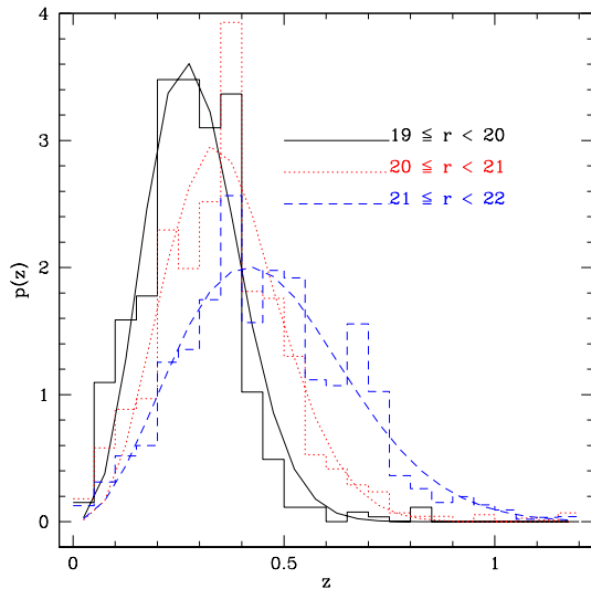
Figure 15. Redshift distributions for all photometric galaxies without lensing selection.
