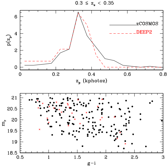
Figure 11. Photoz distribution (top) and colour-magnitude information for DEEP2 and zCOSMOS sources with 0.3 \leq z_s < 0.35 (kphotoz). In the bottom panel, we show the g-i colour and r -band magnitude, where the red crosses are DEEP2 and the black hexagons are zCOSMOS.
