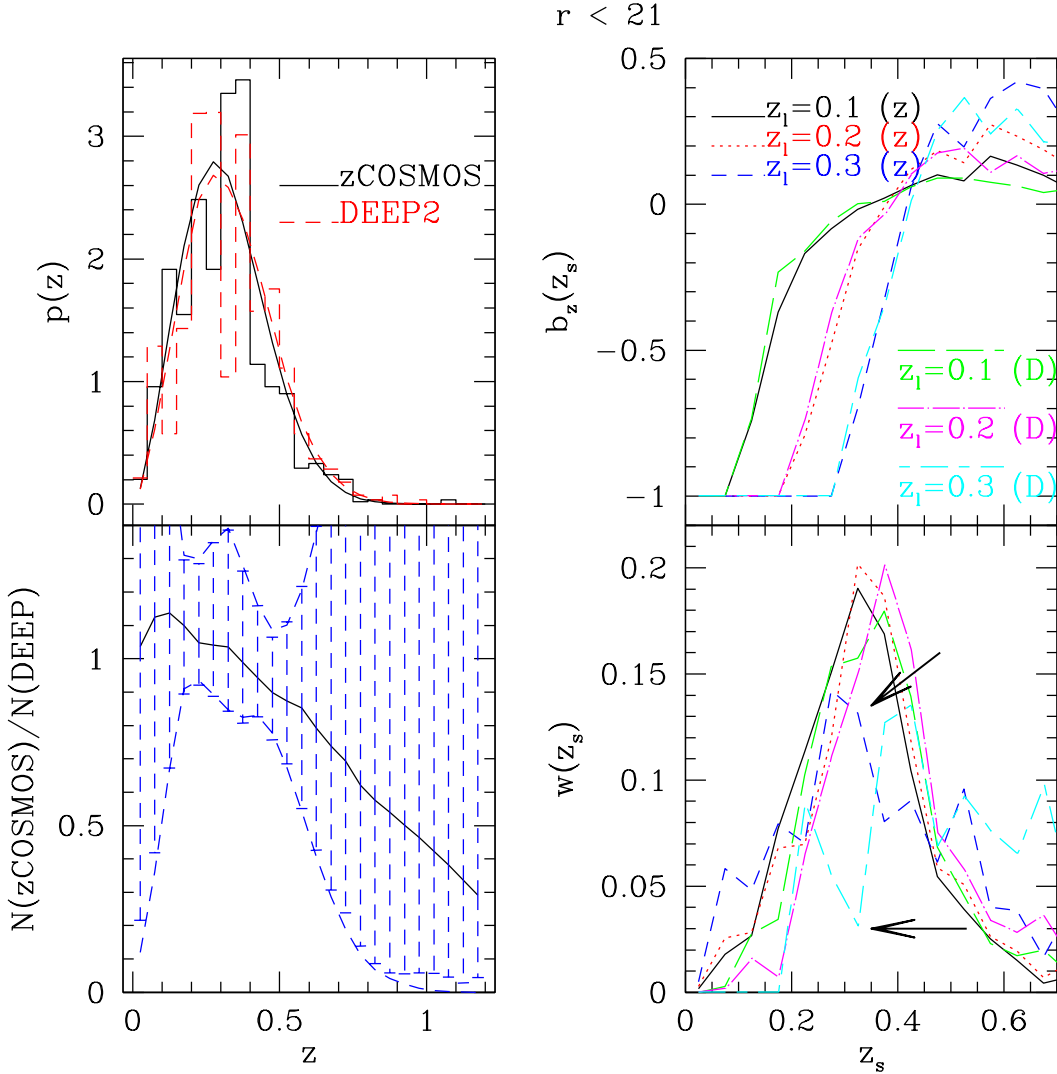
Figure 10. Results for r < 21 only for each survey separately, as described in more detail in the text of section 5.6. We show the best-fit and observed redshift histograms (upper left); the ratio of the best-fit redshift distributions, with shaded 68% CL region (lower left); and the lensing calibration bias b_z (upper right) and the lensing weight as a function of source redshift (lower right) for three lens redshifts.
