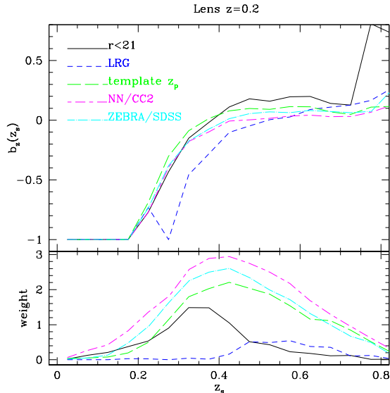
Figure 8. Redshift bias b_z(z_s) (top) and weight (bottom, arbitrary units) for fixed z_l = 0.2 with many methods of source redshift determination as described in the text. Errorbars are not shown here to make the plot simpler to read.
