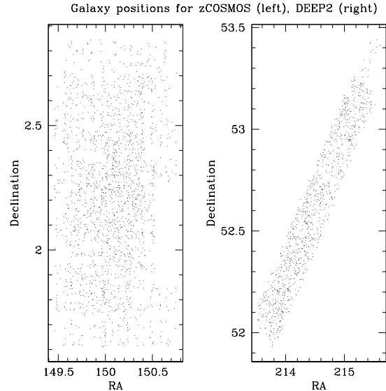
Figure 1. Positions of the zCOSMOS (left) and DEEP2 (right) spectroscopic galaxies used in this work.
