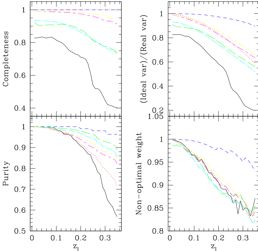
Figure 13. Left: Completeness (top) and purity (bottom) as defined in the text as a function of lens redshift. Top right: The resulting ratio of ideal to real variance for each method of source redshift determination. Bottom right: the derived change in variance due to the non-optimal weighting. Redshift determination methods are as follows: solid black = kphotoz ( r < 21 ), dotted red = r > 21 redshift distribution, dashed blue = high-redshift LRGs, long-dashed green = template photoz’s, long-short-dashed magenta = NN/CC2 photoz’s, long-short-dashed yellow = NN/D1 photoz’s, and dot-dashed cyan = ZEBRA/SDSS.
