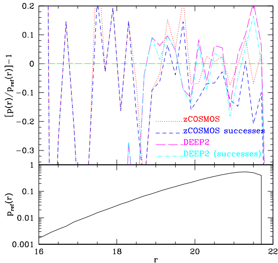
Figure 3. Bottom: r -band apparent magnitude histogram for the full source catalog. Top: Difference between the apparent magnitude histogram for the zCOSMOS and DEEP2 samples relative to that for the full source catalog.
