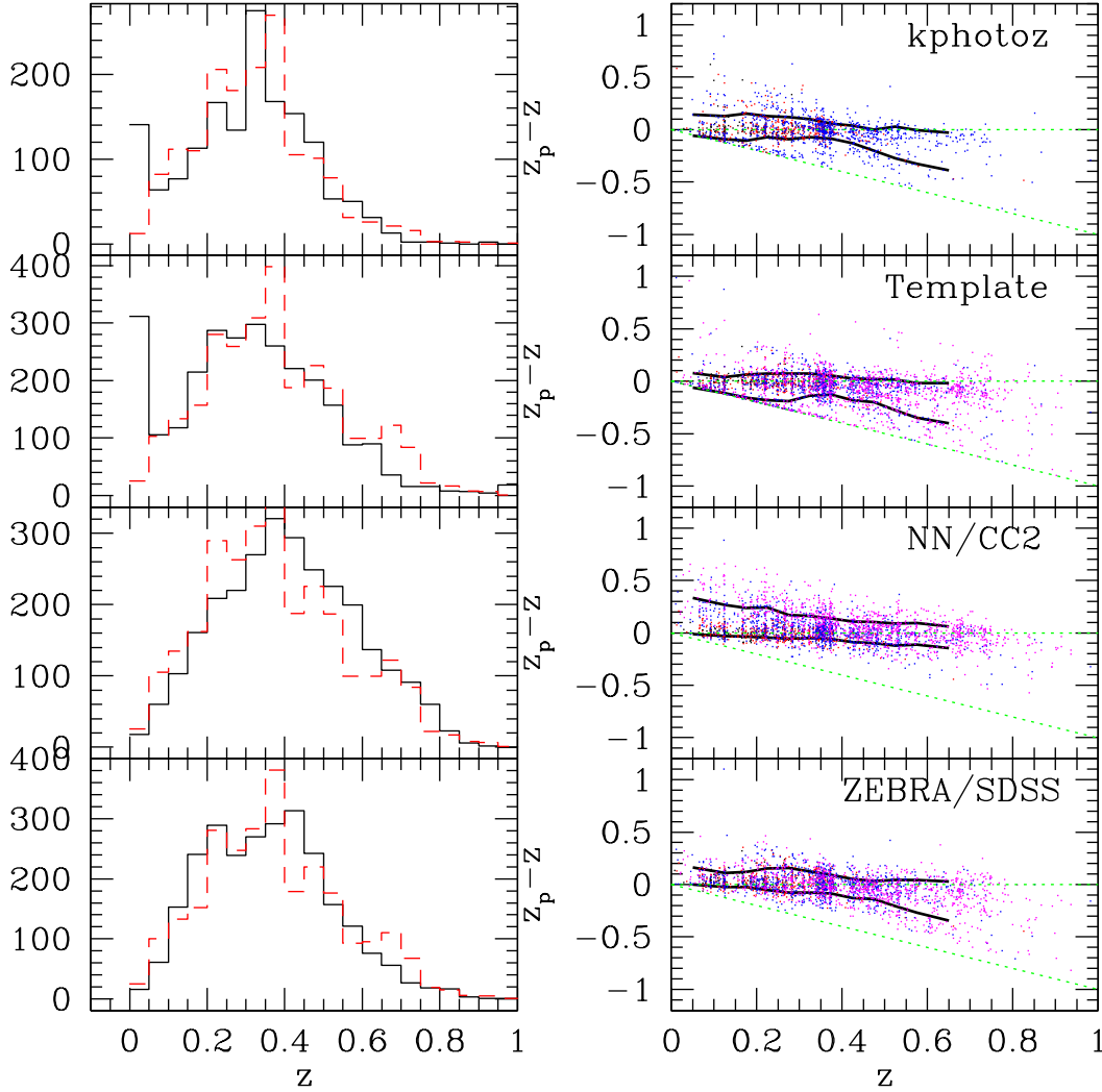
Figure 6. Photometric redshift errors for the photoz methods described in the text (right), and the corresponding redshift histograms (left). In the right panel, the points are coloured according to their apparent magnitude: black for r < 19 , red for 19 \leq r < 20 , blue for 20 \leq r < 21 , and magenta for 21 \leq r < 21.8 . The 68% confidence level limits on the photometric redshift error, determined in bins of \Delta z = 0.05 , are shown as solid lines on the plot (dashed lines show zero error and the lower limit on the error given that z_p > 0 ). In the left panel, the dashed red lines are the true redshift histogram for the galaxies used for the calculation, and the solid black lines are the photometric redshift histograms.
