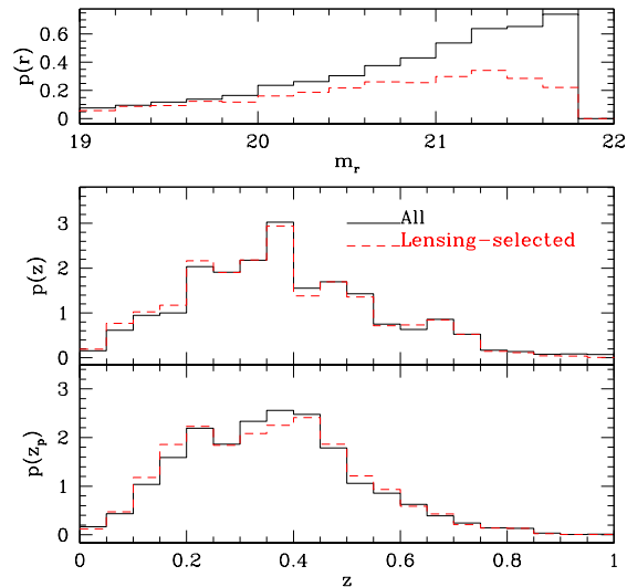
Figure 16. Magnitude (top), redshift (middle), and ZEBRA/SDSS photoz (bottom) histograms for the full flux-limited sample and for the lensing sources. For the magnitude histogram, we have normalized both to the same number of galaxies so the fraction that pass our cuts as a function of magnitude will be apparent. For the redshift and photoz histograms, the histograms for both the full and the lensing-selected sample are normalized to integrate to unity.
