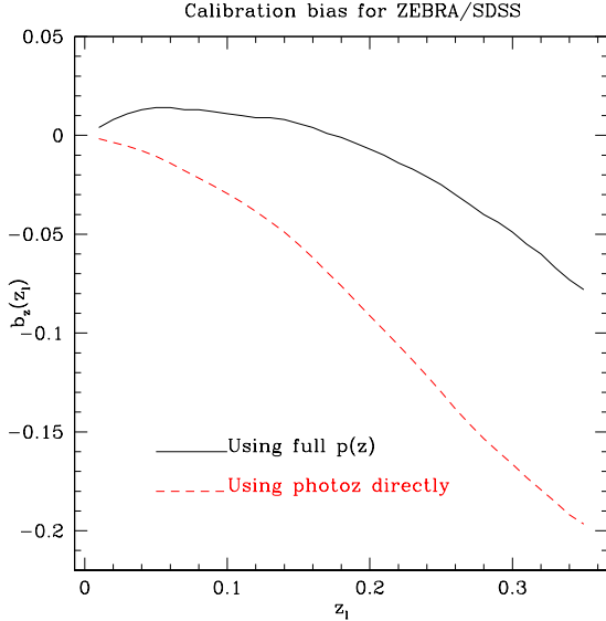
Figure 14. Lensing calibration bias \langle b_z(z_l) \rangle for the ZEBRA/SDSS method, using the photoz directly versus using the full posterior p(z) to compute \Sigma_c as described in the text.
