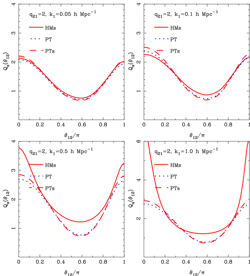
FIG. 2: Comparison of analytic model predictions with results from PT. The configuration dependence is shown for triangles with k_2/k_1 = 2 and on scales: k_1 = \{0.05, 0.1, 0.5, 1.0\} h \text{ Mpc}^{-1} . In all panels: solid (red) lines represent redshift space halo model predictions (HMs); dash (red) lines correspond to redshift space tree-level PT (PTs) [35]; and dotted (blue) lines correspond to real space tree-level PT.
