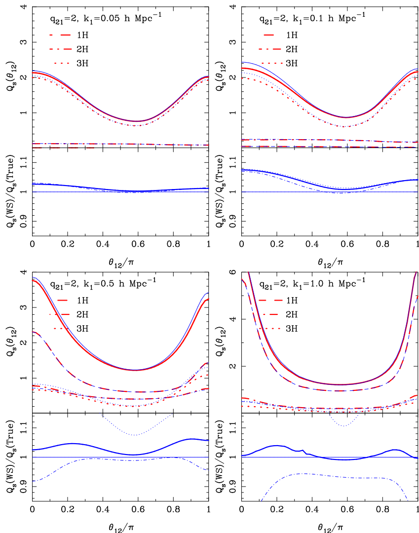
FIG. 1: Configuration dependence of the reduced bispectrum monopole in redshift space – comparison of the predictions from the exact Halo Model expressions with those under the WS-approximation. Top sections of each panel show results for triangles with k_2/k_1 = 2 and on scales: k_1 = \{0.05, 0.1, 0.5, 1.0\} h \text{ Mpc}^{-1} . The dash, dot-dash and dotted lines in each panel correspond to the 1-, 2- and 3-Halo terms, respectively. The solid lines correspond to the sum. Thick (red) and thin (blue) lines are the exact Halo Model and WS approximate results, respectively. Bottom sections of each panel show the ratio of the total WS approximate bispectra to the exact Halo Model calculation. Line styles have same meaning as in top panels.
