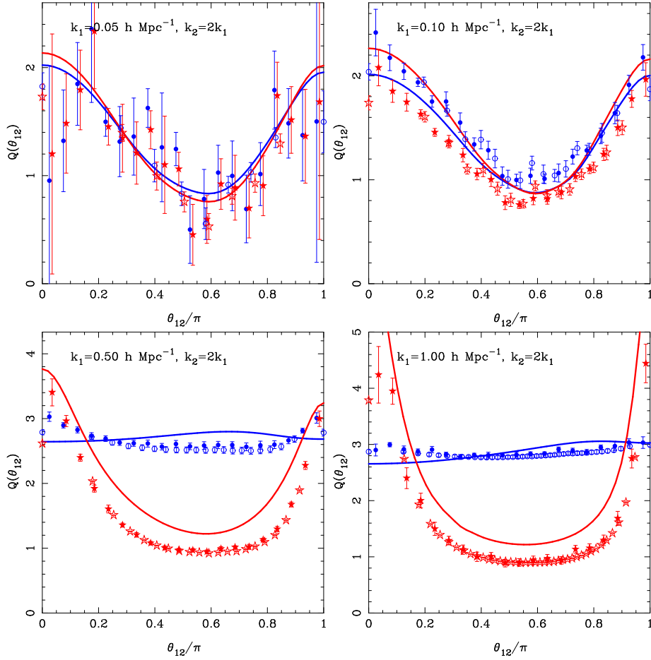
FIG. 7: Comparison of the reduced bispectrum estimates obtained from the method presented in Sec. VIC with those obtained from the “full sampling code” of [88]. As in Fig. 5, our results are represented by solid symbols, and those from the alternate method are denoted by open symbols. Again, errors are on the mean and real and redshift space estimates from the same code have been slightly offset in the x -axis to enhance clarity.
