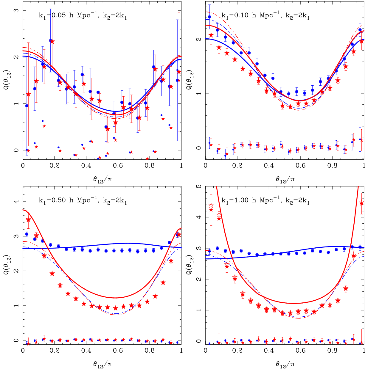
FIG. 5: Same as Fig. 4 only this time for the reduced bispectrum. Additionally, where visible the open symbols represent the shot noise corrected estimates.
