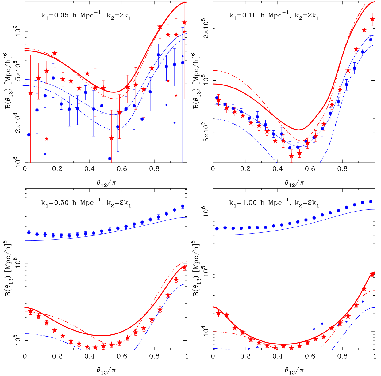
FIG. 4: Configuration dependence of the bispectrum in real and redshift space measured for the dark matter particles in the ensemble of LCDM simulations. The four panels show the configuration dependence for k -space triangles with k_2/k_1 = 2 and for scales k_1 = \{0.05, 0.1, 0.5, 1.0\} h\text{Mpc}^{-1} . Red and blue colors distinguish between real and redshift space quantities. The solid points with error bars show measurements: large solid points are for the real (dots) and redshift space (stars) monopole bispectra; the corresponding smaller points are the imaginary bispectra (which should be zero). The solid lines show the predictions from HM (thin) and HMs (thick). The triple dot-dash lines show the predictions from PT (thin) and PTs (thick). In the top left panel, for clarity we have suppressed the errors on the imaginary bispectra.
