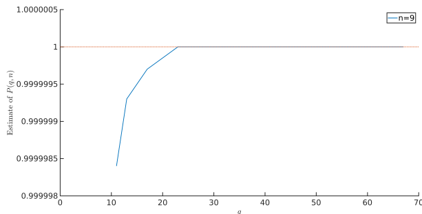
Fig. 2: Estimate of \mu(\tilde{P}_H(q, 9)) obtained from Monte-Carlo tests on 10^7 weight two matrices
