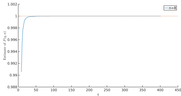
Fig. 1: Estimate of \mu(\tilde{P}_H(q, 8)) obtained from Monte-Carlo tests on 10^7 weight two matrices
