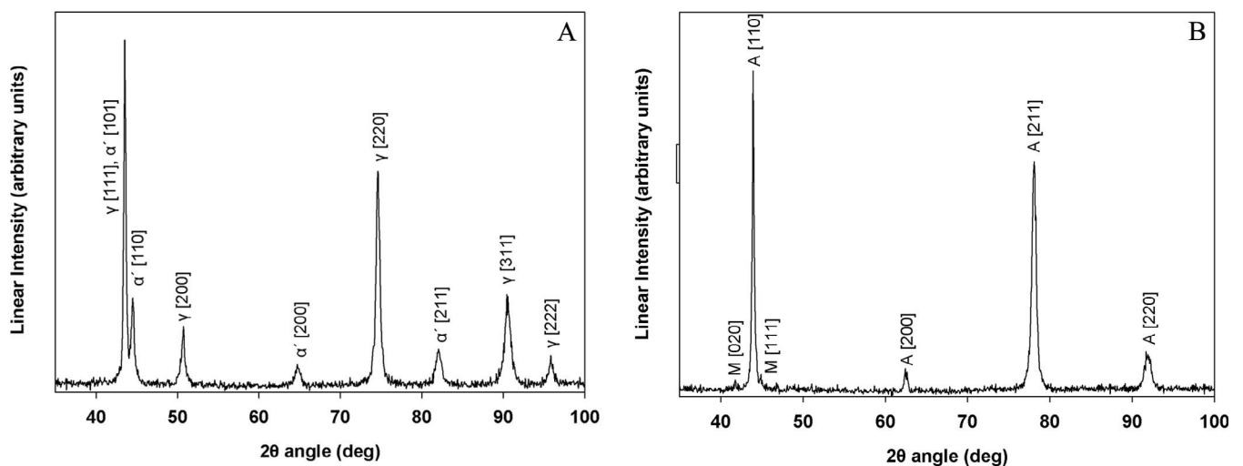
Figure 2. XRD spectra of SAW (A) and NSE (B) wires tested. (A) SAW consists of austenite ( \gamma phase) and martensite ( \alpha' phase) iron structure. (B) NEO shows the presence of NiTi austenite (A) structure with limited presence of martensite (M).
