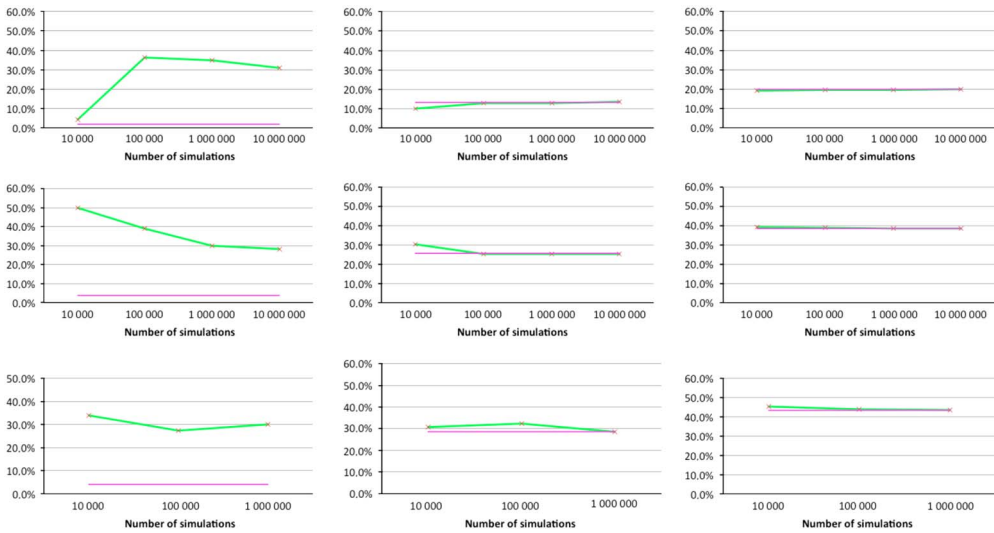
Figure 2. Convergence of the diversification benefit of S_n (associated with TVaR at 99.5%) for \alpha=1.1, 2, 3 (from left to right), for an aggregation factor n=2, 10, 100 (from up to down). The purple lines are for the analytical values and the green ones are the average values obtained from the Monte Carlo (MC) simulations. The y-scale is the same for all the graphs, for fair comparison.
