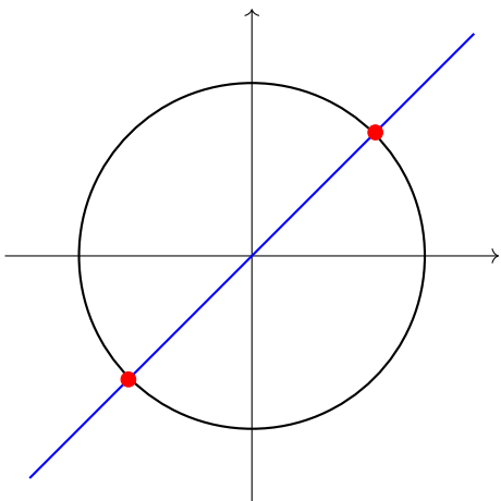
Figure 1. For every vector \mathbf{h} \in \mathbb{R}^2 \setminus \{0\} , the linear subspace \mathcal{T}_{\mathbf{h}} := \{\mathbf{h}z : z \in \mathbb{R}\} intersects the unit circle \mathcal{S}_1 in the two antipodal points \pm \mathbf{h}/\|\mathbf{h}\|_2 .
