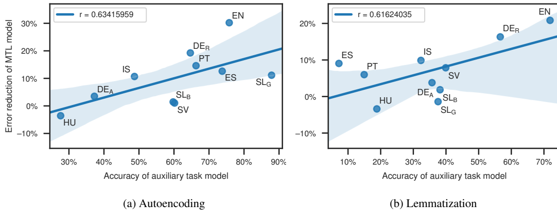
Figure 6: Correlations (with 95% confidence intervals) between the performance of an auxiliary task model applied to normalization data and the error reduction when using this task in a multi-task learning setup.
