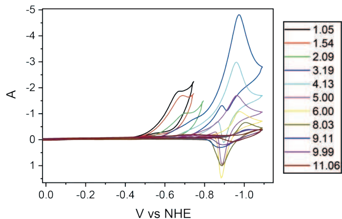
Fig. 1. Cyclic voltammetry on [\text{Co}^{\text{II}}(\text{BPyPy}_2\text{COH})\text{Br}_2] (1 mM) in 40 mM BRB, 100 mM LiOTf, 100 mV/s, pH adjusted with 2 M NaOH, referenced to NHE with [\text{MVCl}_2] , WE = Hg, CE = Pt, RE = Ag/AgCl.
