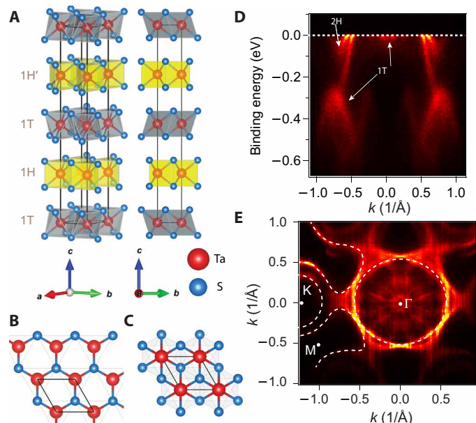
Fig. 1. Structure of 4Hb-TaS 2 . (A) 3D schematic drawing of a unit cell of 4Hb-TaS 2 showing the alternate stacking of octahedral (T) and trigonal prismatic (H) layers. Top views of 1H and 1T layers are shown in (B) and (C), respectively. The top view of the 1H layer displays the in-plane broken mirror symmetry. (D) An ARPES detector image obtained at T = 15 K using 72 eV of photon energy reveals the electronic band structure along the \Gamma -M direction. (E) A Fermi surface mapping under the same conditions. The band structure is a combination of 2H-TaS 2 and CDW reconstructed 1T-TaS 2 , which was rigidly shifted toward the Fermi level [horizontal white dashed line in (D)]. The dashed line represents the 2H-TaS 2 Fermi surface.
