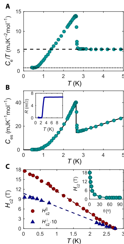
Fig. 2. Specific heat and transport measurements. (A) The electronic contribution to the heat capacity divided by the temperature C_e/T is plotted as function of T . The dashed line represents the total electronic specific heat in the normal state, and the dotted line is a residual linear contribution coming from the 1T layers (see the main text for details). (B) The electronic-specific heat after the removal of the 1T contribution displaying a BCS-type behavior with \Delta = 0.4 meV. Inset: Resistance versus temperature shows enhanced T_c . (C) H_{c2} as a function of temperature for in-plane (red circles) and out-of-plane (blue triangles) field orientations. For better visibility, H_{c2} is multiplied by 10. Inset: The angular dependence of H_{c2} showing strong anisotropy.
