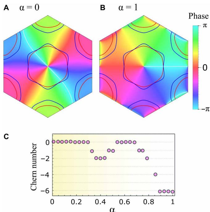
Fig. 4. Superconducting order parameter. (A) and (B) show the phase of the gap functions e_{\mathbf{k}} and o_{\mathbf{k}} , respectively, superimposed on the Fermi surface of 1H-TaS 2 . (C) The corresponding Chern number as a function of the mixing parameter \alpha appearing in Eq. 2. Note that the values presented here were computed numerically and are not rounded to an integer.
