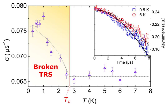
Fig. 3. TRS breaking. A sudden increase in the zero-field muon spin relaxation rate \sigma is observed at T_c (marked by the vertical line), marking the onset of TRS breaking. The dotted line is a guide to the eye. The inset shows two ZF- \mu\text{SR} spectra at different temperatures, above and below T_c . The black lines are best fits to Eq. 1.
