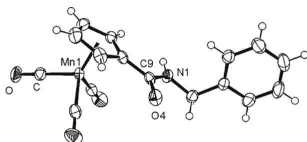
Figure 2. ORTEP presentation of [(\text{Cp-ba})\text{Mn}(\text{CO})_3] 5a . Important bond lengths (Å) and angles ( ^\circ ) are: Mn(1)-C(1) = 1.7905(16); Mn(1)-C(3) = 1.796(2); Mn(1)-C(2) = 1.7996(17); Mn(1)-C(4) = 2.1210(15); Mn(1)-C(5) = 2.1363(16); C(9)-N(1) = 1.339(2); C(10)-N(1) =
