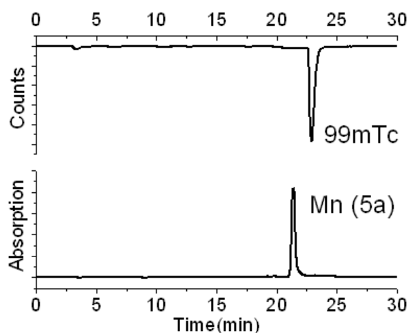
Figure 3. HPLC trace of the cold manganese complex 5a and the corresponding ^{99m}\text{Tc} complex 6a complex as prepared directly from [^{99m}\text{TcO}_4] . The time difference is due to detector separation.
