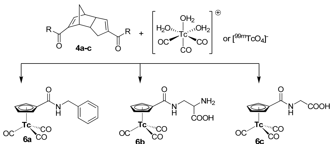
Scheme 3. Preparation of the ^{99\text{mTc}} complexes 6a-c under aqueous conditions.
