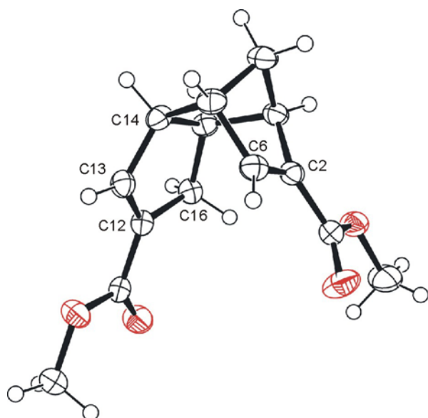
Figure 1. ORTEP presentation of Thiele's acid dimethyl ester. Important bond lengths (Å) and angles (°) are: C(2)-C(6) = 1.3374(19); C(12)-C(16) = 1.5009(18); C(12)-C(13) = 1.3343(17); C(13)-C(14) = 1.4947(17); C(6)-C(2)-C(1) = 124.76(12); C(6)-C(2)-C(3) = 107.74(11); C(13)-C(12)-C(11) = 126.00(12); C(13)-C(12)-C(16) = 113.05(11); C(12)-C(13)-C(14) = 112.40(11).
