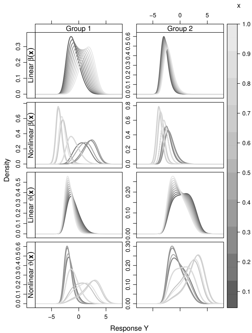
Fig. 1 Artificial Data-generating Processes (DGPs). Conditional densities given two groups (left and right panel) and x \in [0, 1] (gray color coding) for four different data-generating processes.
