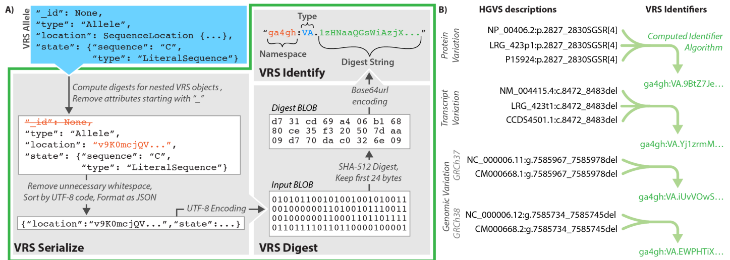
Figure 4 - Computed identifiers
