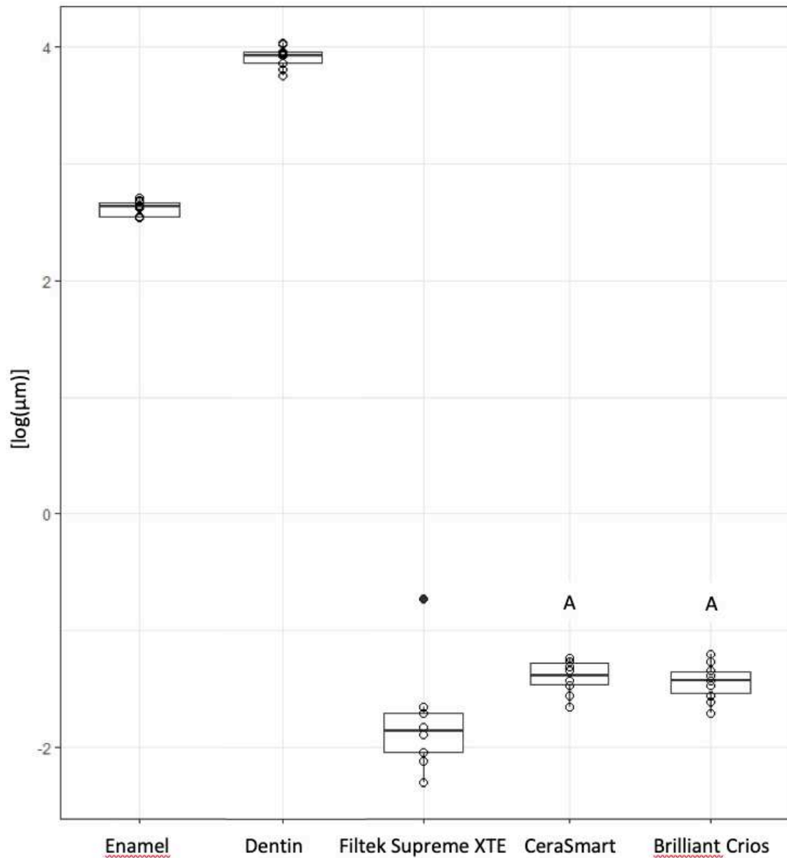
Figure 2: Erosive/abrasive wear [ \mu\text{m} ] in logarithmic form of the five materials under investigation. The boxes represent the 25 th and 75 th percentile, respectively. The center line indicates the median and the circles represent the respective mean values per sample. Only the CeraSmart and Brilliant Crios groups do not differ significantly from each other. Box plots marked with the same letter, do not differ significantly from each other.
