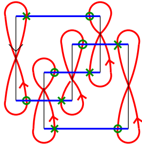
Figure 2: Oriented figure-eights and particular elements \mathbf{x} and \mathbf{o} of \mathcal{G}
