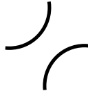
Figure 16: Resolution used in the definition of Khovanov homological grading on \mathcal{H}
