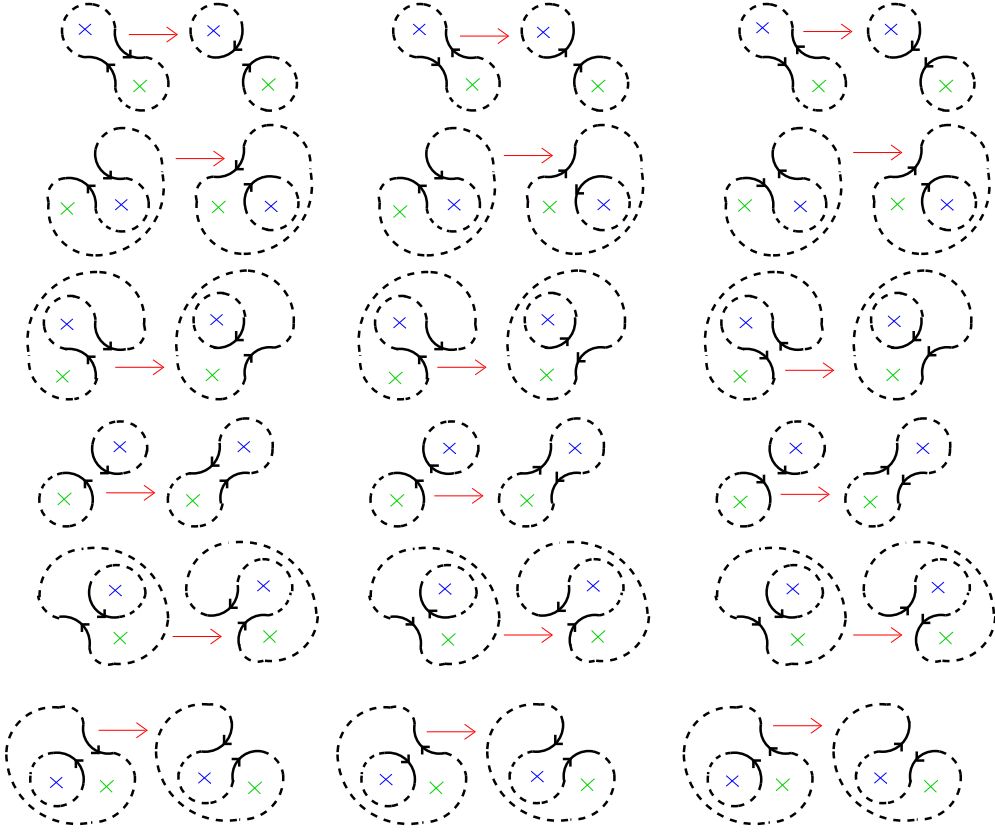
Figure 26: Non-zero differentials in Khovanov complex
