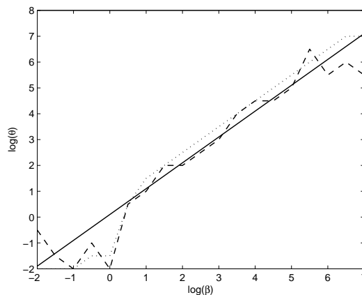
Figure 2: Simulated optimal taper values \theta as a function of \beta in (natural) log-scale. For q = 40 and n = 10 , p(h) = \exp(-3h/\beta) and c(h) = \exp(-3h/\theta) . The approximation given by (22) (solid) follows closely the optimal values of \theta minimizing \|\mathbf{P}^f - \hat{\mathbf{P}}_{\mathbf{C}}^f\|_{\mathbb{E}}^2 (dashed) and \|\mathbf{P}^a - \hat{\mathbf{P}}_{\mathbf{C}}^a\|_{\mathbb{E}}^2 (dotted). (See Section 6 for the simulation setup.)
