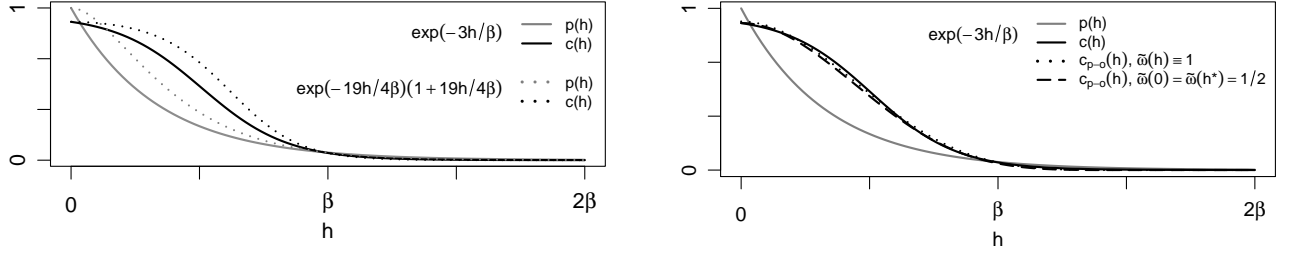
Figure 3: Left panel: Covariance functions and optimal tapers based on (20). The exponential covariances p(h) = \exp(-3h/\beta) (solid) and p(h) = \exp(-19/4 \cdot h/\beta)(1 + 19/4 \cdot h/\beta) (dotted) are depicted in gray (lower curves). For n = 20 , the optimal tapers c(h) are depicted in black (top curves). Right panel: For n = 20 , the optimal taper c(h) (solid black) for the exponential covariance p(h) = \exp(-3h/\beta) (solid gray), along with compactly supported covariance functions given by Gaspari and Cohn (1999). The pseudo-optimal taper functions are fitted using (24) by matching the sill and effective range of c(h) (dashed) and by using a constant weight function \tilde{\omega}(h) (dotted).
