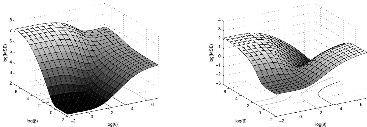
Figure 8: \log(\|\mathbf{P}^f - \hat{\mathbf{P}}_C^f\|_E^2) (left panel) and \log(\|\mathbf{P}^a - \hat{\mathbf{P}}_C^a\|_E^2) (right panel) as a function of the covariance parameter \beta and the tapering parameter \theta (note the log-scales). Here, q = 40 and n = 10 . The contours along large values of \theta give the MSEs associated with un-tapered \hat{\mathbf{P}}^f (see Table 1). For both \hat{\mathbf{P}}_C^f and \hat{\mathbf{P}}_C^a , the optimal taper values track along the contour \log(\theta_{\text{opt}}) \approx \log(\beta) (see also Figure 2).
