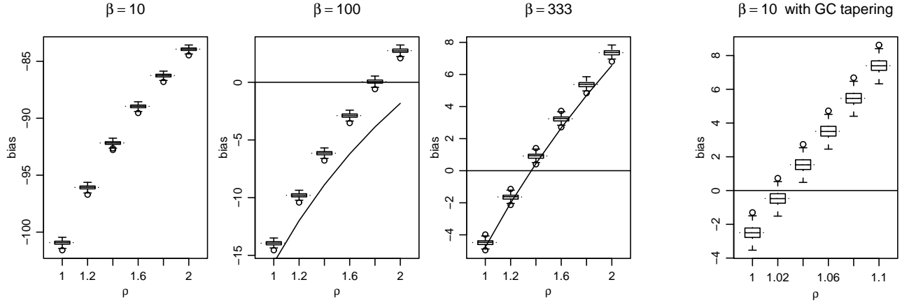
Figure 9: Boxplots of \text{tr}(\hat{\mathbf{K}}_\rho - \mathbf{K}) . Left panel: The bias for different inflation factors \rho and parameters \beta . Here, \hat{\mathbf{K}}_\rho is based on the tapered and boosted forecast covariance \rho\hat{\mathbf{P}}^f and n = 10 . The superimposed solid line represents the second order approximation given by (26). Right panel: For \beta = 10 , \hat{\mathbf{K}}_\rho is based on the tapered and boosted forecast covariance \rho\hat{\mathbf{P}}_C^f . The means are dotted.
