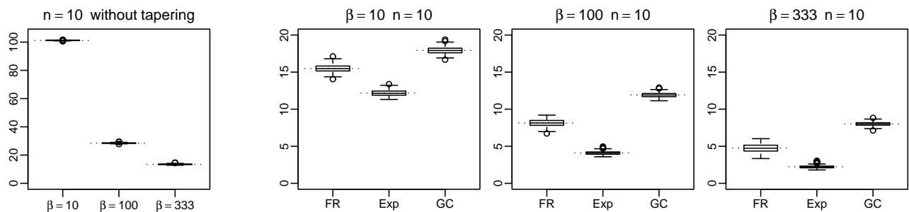
Figure 7: Box-plots of simulated values of \|\mathbf{P}^a - \hat{\mathbf{P}}_C^a\|^2 . Left panel: un-tapered squared errors \|\mathbf{P}^a - \hat{\mathbf{P}}^a\|^2 . Right panel: tapered squared errors \|\mathbf{P}^a - \hat{\mathbf{P}}_C^a\|^2 as a function of \beta and the choice of taper function. Each plot is based on 100 simulations and n = 10 . The means are dotted. Note the difference in scale in the left and right panels.
