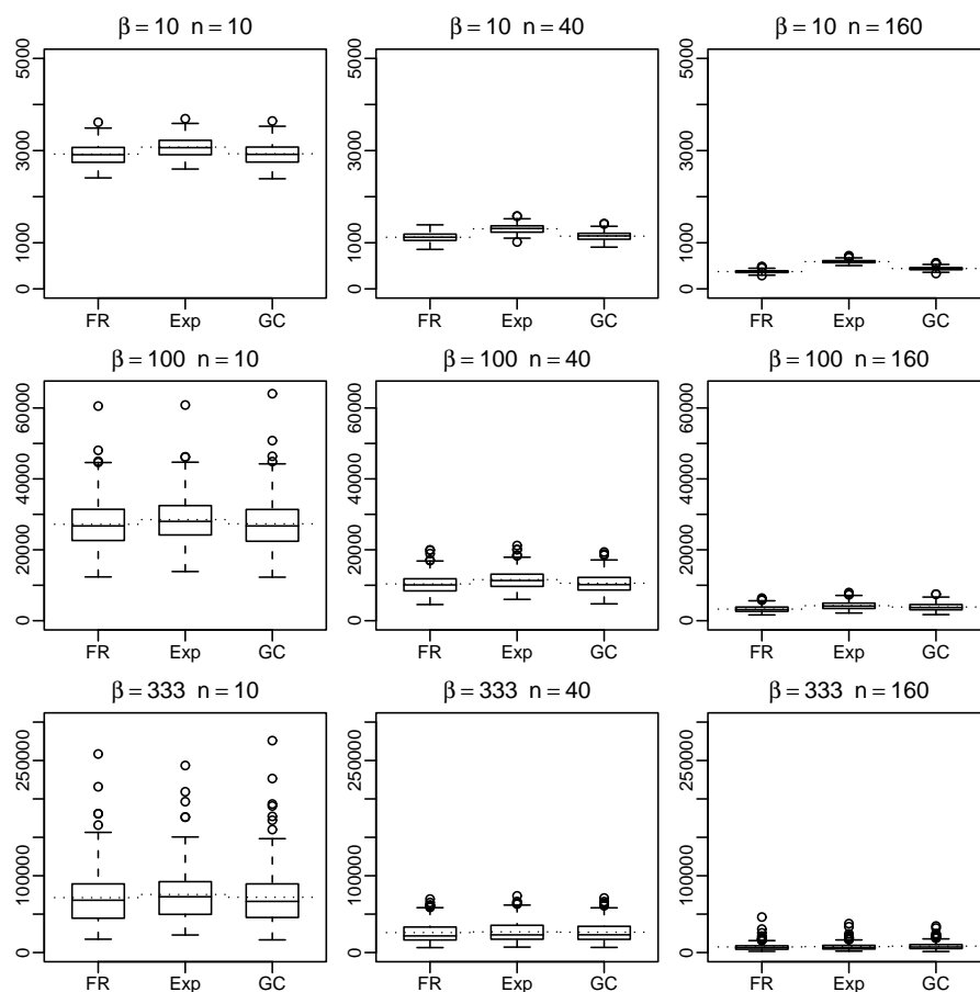
Figure 5: Box-plots of simulated values of \|\mathbf{P}^f - \hat{\mathbf{P}}_C^f\|^2 . The rows correspond to range parameters \beta = 10, 100 , and 333 , and the columns to ensemble sizes n = 10, 40 and 160 . For each of the nine plots, the relative effectiveness of the taper variants (FR, Exp, GC) may be assessed through comparison of side-by-side box-plots. The means are dotted.
