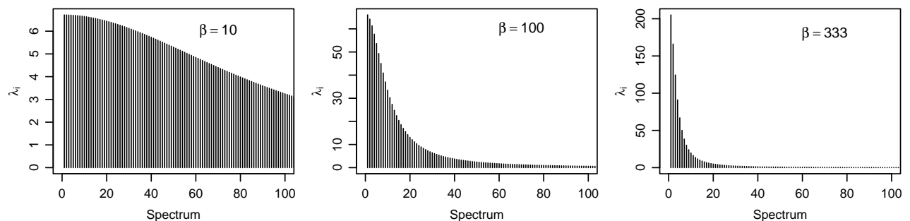
Figure 4: The eigen-spectrum of the forecast covariance matrix used in the simulations. Here, \mathbf{P}^f is based on the exponential covariance function p(h) = \exp(-3h/\beta) . The three plots show the first 100 modes of \mathbf{P}^f for \beta = 10 (left), \beta = 100 (middle), and \beta = 333 (right).
