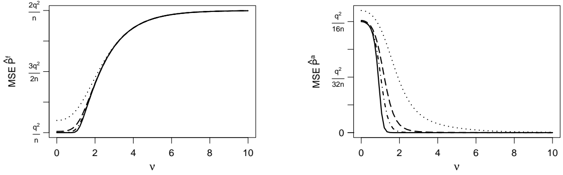
Figure 1: Left panel: \|\mathbf{P}^f - \hat{\mathbf{P}}^f\|_{\mathbb{E}}^2 evaluated through (12) as a function of the decay rate of the eigen-structure of \mathbf{P}^f . The i th eigenvalue of \mathbf{P}^f is given by \lambda_i = ci^{-\nu} , with c chosen such that \text{tr}(\mathbf{P}^f) = \text{tr}(\mathbf{R}) = q . The four curves in each plot correspond to q = 10 (dotted), q = 10^3 (dashed), q = 10^6 (dash-dotted), and q \rightarrow \infty (solid). Right panel: Lower bound of \|\mathbf{P}^a - \hat{\mathbf{P}}^a\|_{\mathbb{E}}^2 evaluated through the second order approximation (14).
