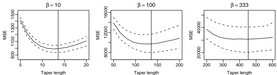
Figure 6: \|\mathbf{P}^f - \hat{\mathbf{P}}_C^f\|^2 as a function of the taper length of a GC-taper for n = 40 . The vertical lines give the optimal taper lengths according (24) with \tilde{\omega}(0) = \tilde{\omega}(h^*) = 1/2 and \tilde{\omega}(h) = 0 otherwise. The dotted lines are point-wise 10 and 90 percent empirical confidence intervals.
