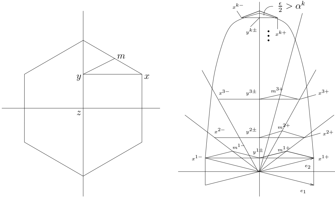
Figure 1. The figure on the left hand side shows the unit sphere of a ball convex but not distance convex Banach space. On the right hand side the construction method of the proof of Proposition 4 is illustrated.
