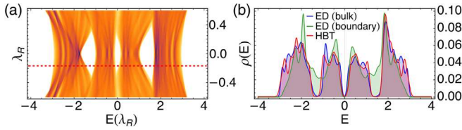
FIG. 3. Hyperbolic Kane-Mele model. (a) Density of states for t_2 = M/2 = \frac{1}{6} computed from HBT, which reveals three energy gaps at small Rashba coupling \lambda_R . (b) Bulk-DOS functions for \lambda_R = -\frac{1}{6} (red dashed line in (a)) computed using HBT (red) and ED (blue), and the boundary-DOS function (green).
