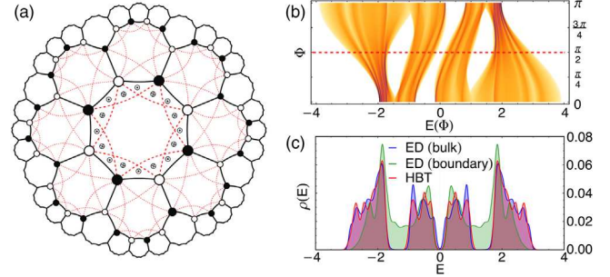
FIG. 2. Hyperbolic Haldane model. (a) Schematic depiction of the model. Red dashed lines indicate next-to-nearest neighbor hopping with amplitude t_2 e^{\pm i\Phi} . The phases \pm\Phi arise due to alternating magnetic fluxes [symbols \odot ( \otimes ) in the innermost octagon] through the system. (b) Density of states for t_2 = M/2 = \frac{1}{6} computed from HBT, revealing three energy gaps. (c) Bulk-DOS functions \rho^{\text{HBT}}(E) and \rho^{\text{ED}}_{\text{bulk}}(E) for \Phi = \pi/2 (red dashed line in b) computed using HBT (red) and ED (blue), and the boundary-DOS \rho^{\text{ED}}_{\text{boundary}} (green).
