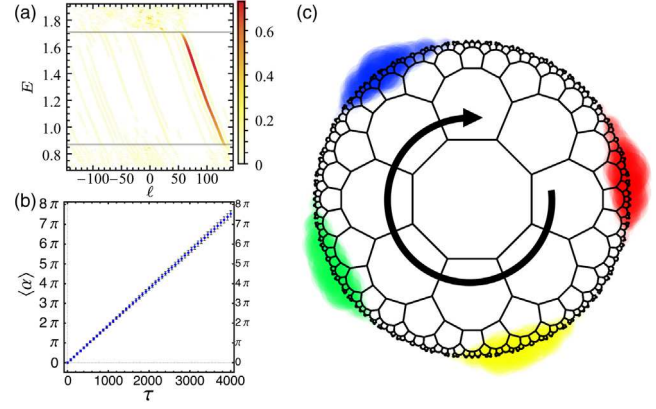
FIG. 4. Topological edge states. (a) Edge-dispersion E as a function of angular momentum \ell for chiral edge states in the upper energy gap of the hyperbolic Haldane model. (b) Propagation of a Gaussian wave packet along the flake boundary; \langle \alpha \rangle is the angular displacement in time \tau , and error bars indicate the width of the wave packet. (c) Snapshots of the wave packet at \tau = 0, 240, 480, 720 (colored, respectively, red, yellow, green, and blue). The area of a disk centered at a given site encodes the probability to find the particle at that site.
