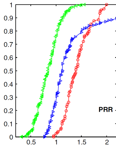
Figure 2: Empirical distribution functions of state-price/state-probability ratios from the experimental session of eight trading periods in Bossaerts et al. (2010) with W_G = 272 , W_B = 162 , and W_R = 81 . The distribution function with circles is for p_R/\pi_R ; the one with arrows pointing to the right is for p_B/\pi_B ; the one with arrows pointing to the left is for p_G/\pi_G . This figure is a copy of Figure 8, right panel, in Bossaerts et al. (2010).
