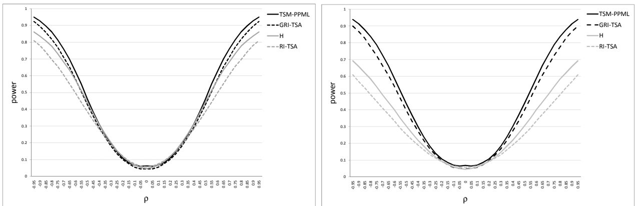
Figure 1: Empirical power of tests for exogeneity
