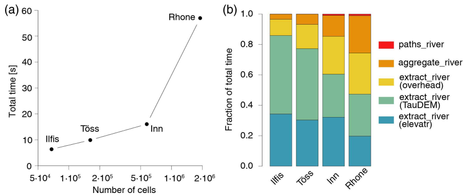
Figure 4. Estimates of computational time needed to produce the river objects used in the analysis of Fig. 3. (a) Total time required as a function of the number of cells in the catchment. (b) Breakdown of time for the different rivnet functions used: in particular, the time spent by extract_river is partitioned into time required by DEM downloading (“ elevatr ”), application of TauDEM commands (“ TauDEM ”) and creation of a river object (“ overhead ”). Results are the average of five runs operated via an Intel ® quad core i7-7700K processor with 16 GB RAM; TauDEM commands were run with eight parallel processors.
