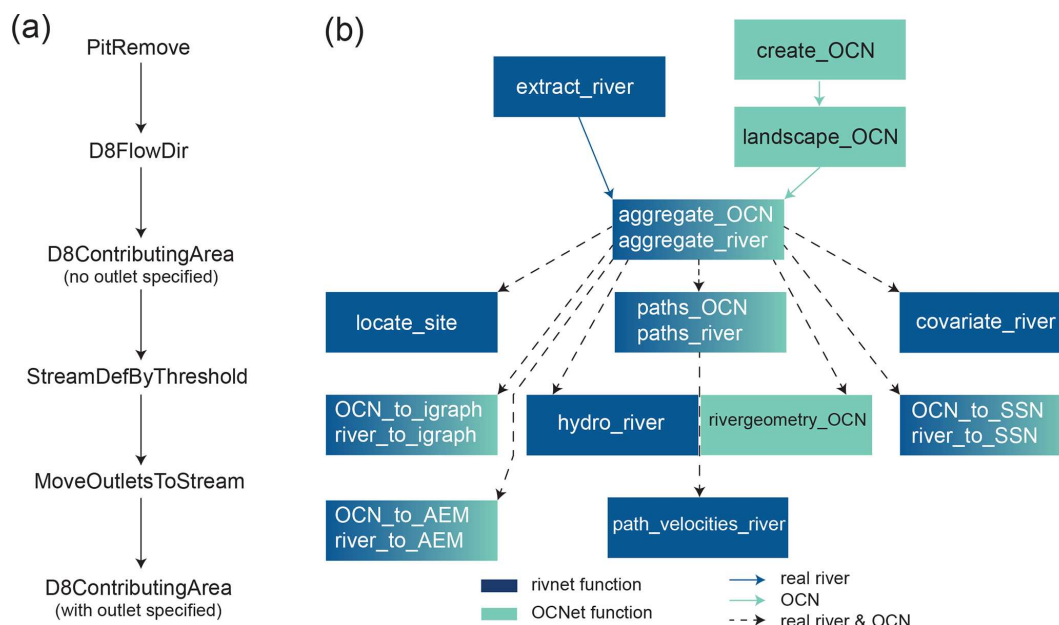
Figure 1. (a) Sequence of TauDEM commands operated by extract_river . (b) Structure of the rivnet and OCNet packages. In both panels, arrows indicate that the output of a function is used as input of the next function.
