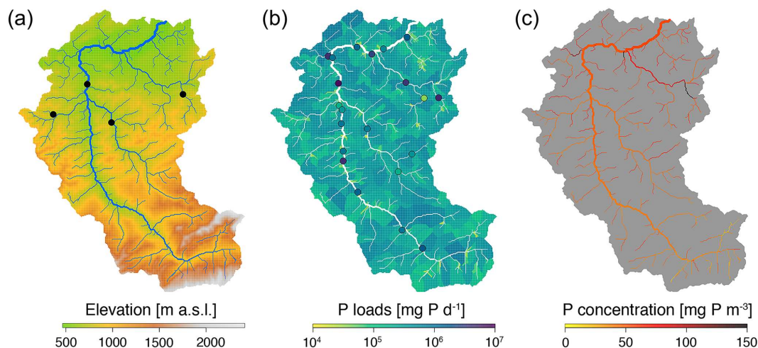
Figure 5. Results of the case study on phosphorous release and transport. (a) Elevation map of the Thur catchment. Black dots indicate the locations of the hydrological stations. (b) Map of phosphorous loads: diffuse loads \phi_{D,i} are color-coded on the respective subcatchments, while point loads \phi_{P,i} are displayed as dots. (c) Map of phosphorous concentration as predicted by the model (Eq. 1). The three panels were obtained as specific cases of the plot() function.
