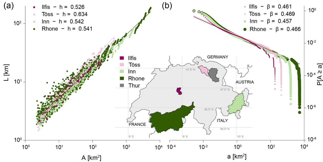
Figure 3. Results of the case study on scaling properties of river networks. (a) Scaling of length of the main river stem L with drainage area A (Hack's law): L \sim A^h . Fitted Hack's exponent values for the four analyzed basins are reported in the legend. (b) Probability distribution of drainage areas P[A \geq a] \sim a^{-\beta} . Fitted exponent values are reported in the legend. The inset displays the location of the four analyzed basins within Switzerland, as well as the Thur catchment (Fig. 5).
