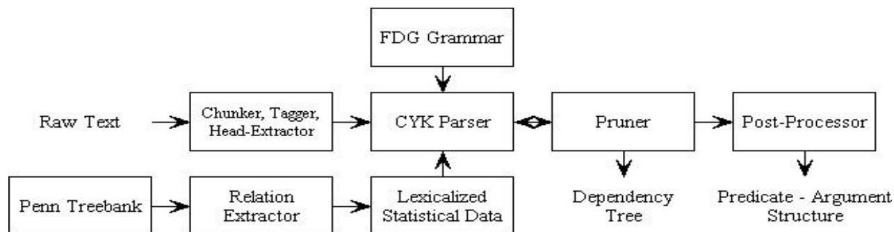
Figure 1: Pro3Gres flowchart
