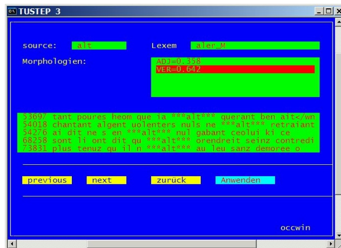
Fig. 1. The Phoenix tool for manual disambiguation
