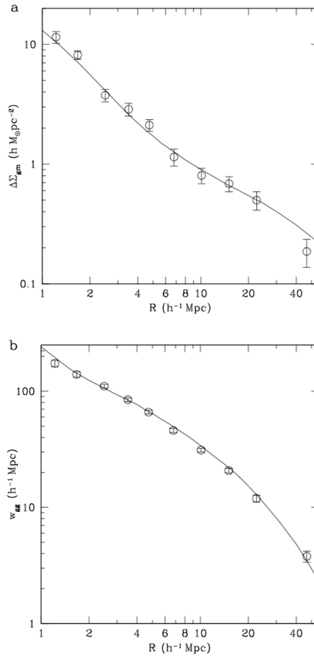
Figure 1 | Probes of large-scale structure measured from ~70,000 luminous red galaxies (LRGs). Observed radial profiles for two complementary probes, galaxy-galaxy lensing (a) and galaxy clustering (b) are shown for scales R = 1.5 - 47h^{-1} Mpc (open circles). The 1\sigma error bars (s.d.) are estimated from jackknife resampling of 34 equal-area regions in the sky. Profiles measured from mock galaxy catalogues are also shown (solid curves).
