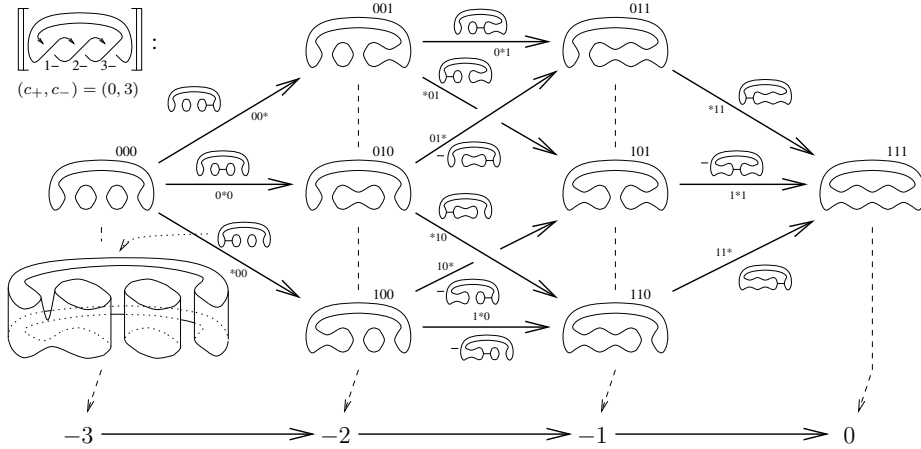
Figure 3. The cube of resolutions for the trefoil.
