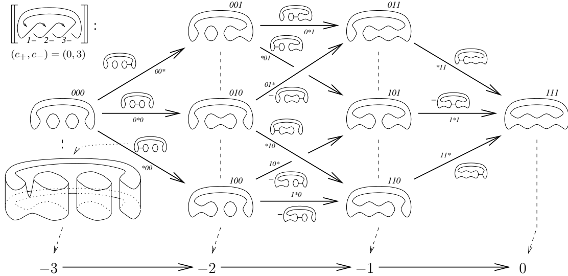
FIGURE 3. The cube of resolutions for the trefoil
