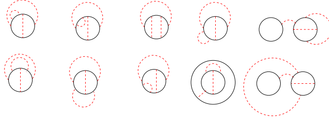
FIGURE 2. Cocycle conditions for \text{NesCob}_1
