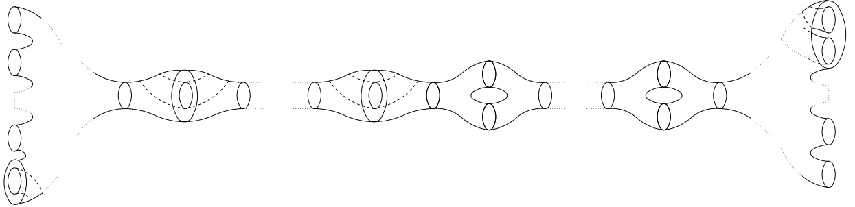
FIGURE 1. Normal form with inner and outer handles
