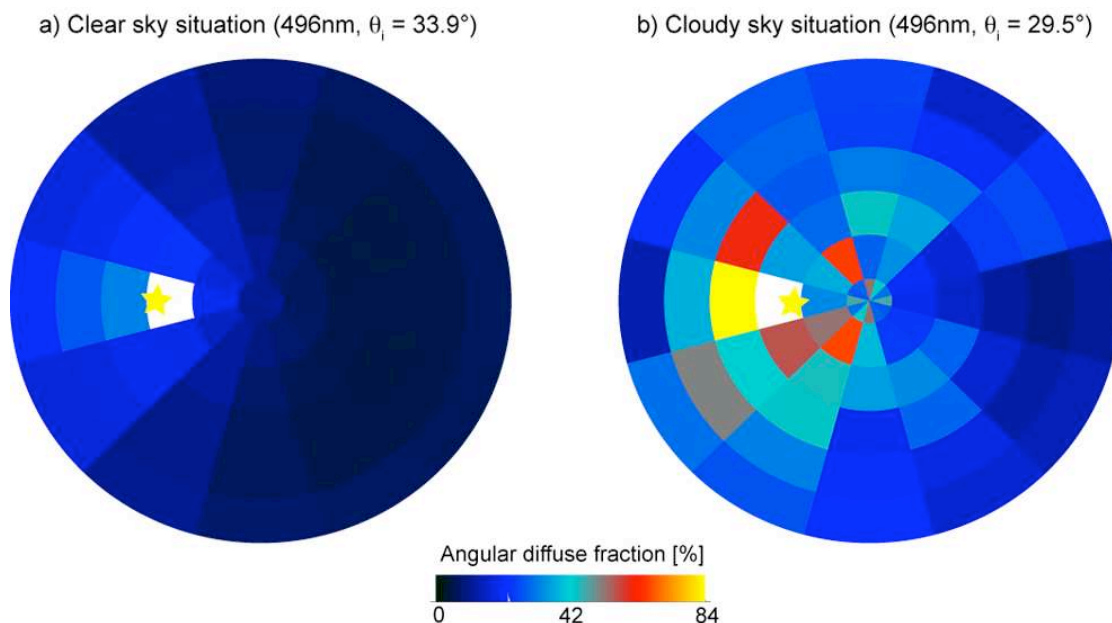
Figure 10. Angular diffuse fraction for different atmospheric situations (clear, cloudy) from dual-view FIGOS measurements (datasets FA9 and FA1). The position of the sun is marked by the sun symbol.
