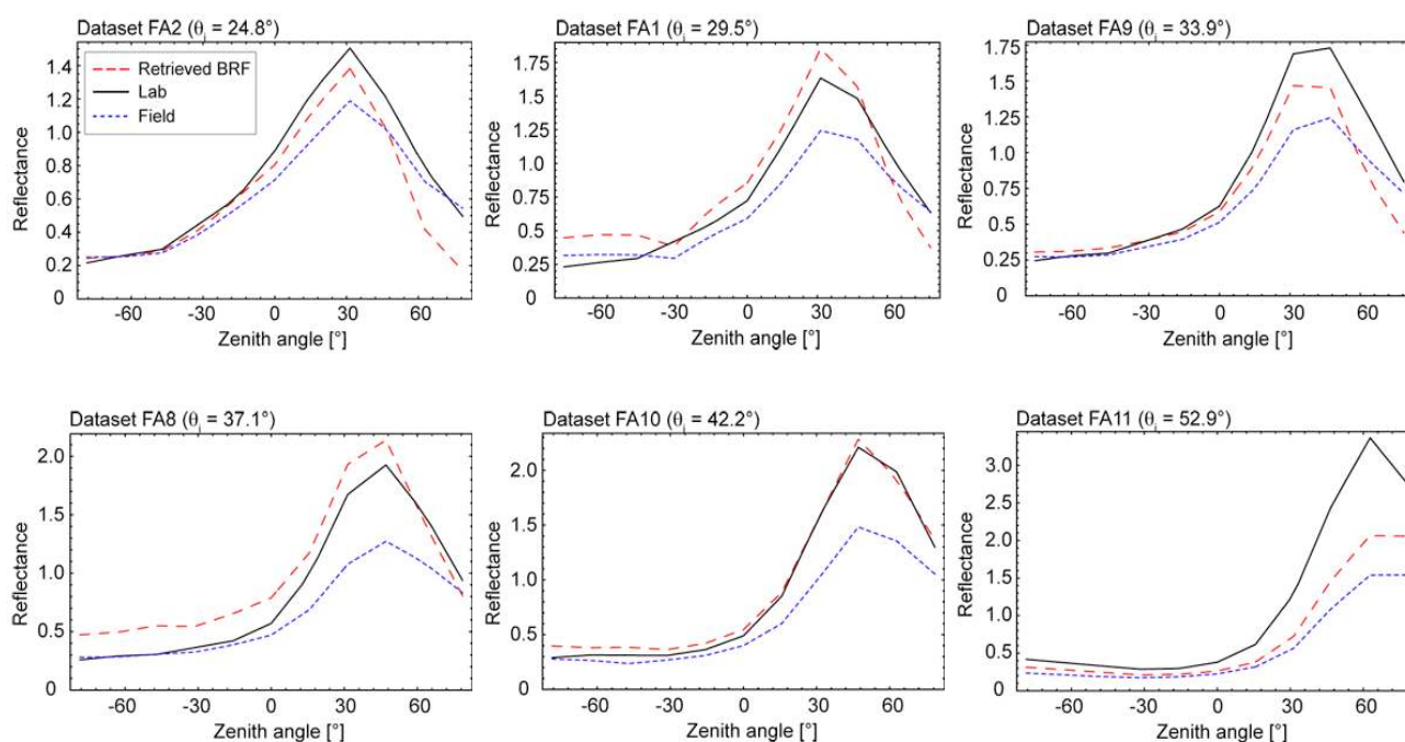
Figure 11. Comparison of BRF retrieval results and spectrodirectional field and laboratory measurements in the principal plane ( -75^\circ backward scattering to 75^\circ forward scattering). The illumination is from the left.
