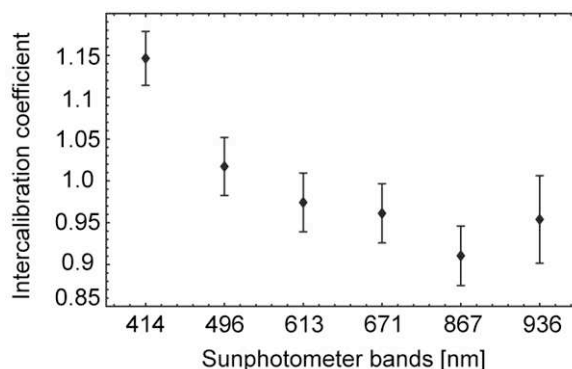
Figure 6. ASD FieldSpec 3 – sunphotometer intercalibration coefficients and respective standard deviation.
