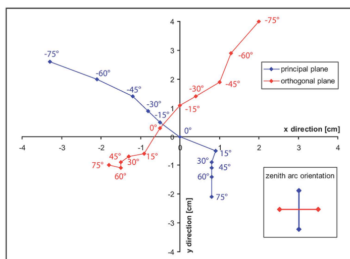
Figure 3. Pointing accuracy over the zenith arc. The convention -x/y and +x/y is used for the backward scattering and the forward scattering direction, respectively. The coordinate system is aligned to the centre of the azimuth arc.
