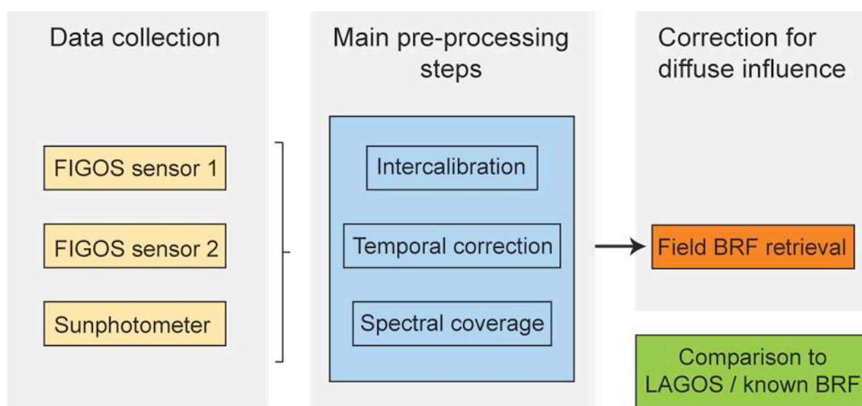
Figure 4. Dataflow scheme for processing dual-view FIGOS datasets.
