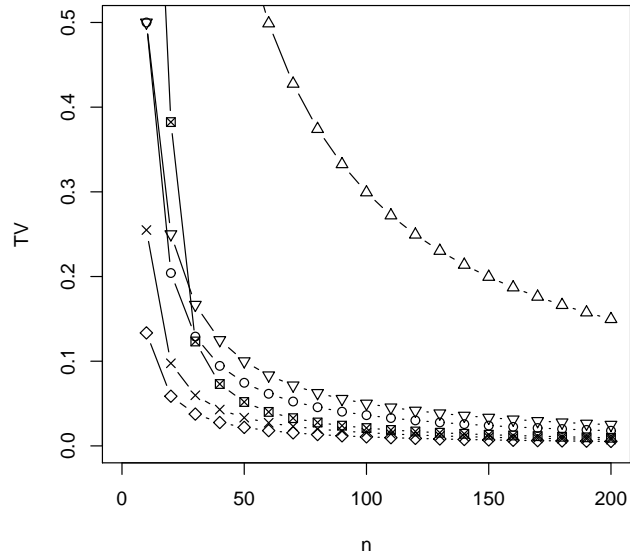
Figure 2: Bounds on the total variation distance d_{TV}(C_Q\text{Bin}(p, Q), \text{CPo}(\lambda, Q)) for Q \sim \text{Geom}(\alpha) as in Figure 1, here plotted against the parameter n , with \alpha = 0.2 and \lambda = 5 fixed.
