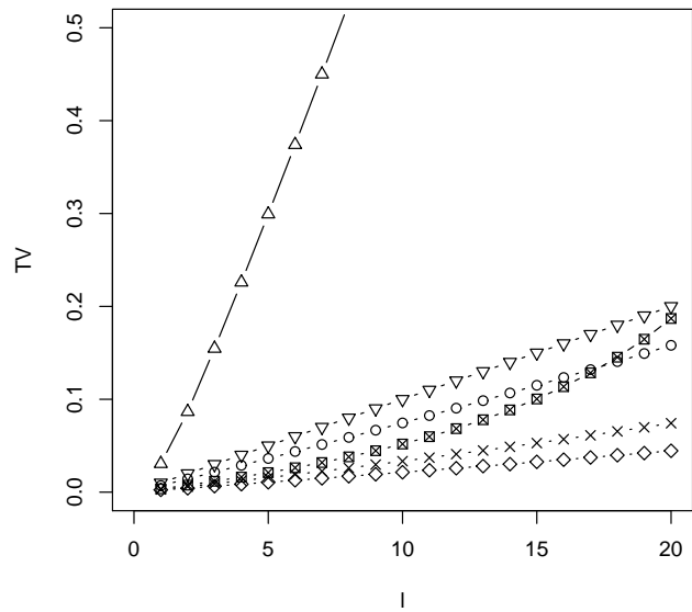
Figure 3: Bounds on the total variation distance d_{TV}(C_Q\text{Bin}(p, Q), \text{CPo}(\lambda, Q)) for Q \sim \text{Geom}(\alpha) as in Figure 1, here plotted against the parameter \lambda , with \alpha = 0.2 and n = 100 fixed.
