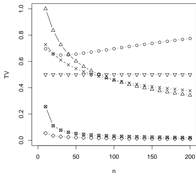
Figure 5: Bounds on the total variation distance d_{TV}(P_{S_n}, \text{CPo}(\lambda, Q)) for Q_i \sim \text{Geom}(\alpha_i) as in Figure 4, where \alpha_i are uniformly spread between 0.15 and 0.25, n varies, and p is as in Regime II, p = \sqrt{0.5/n} .
