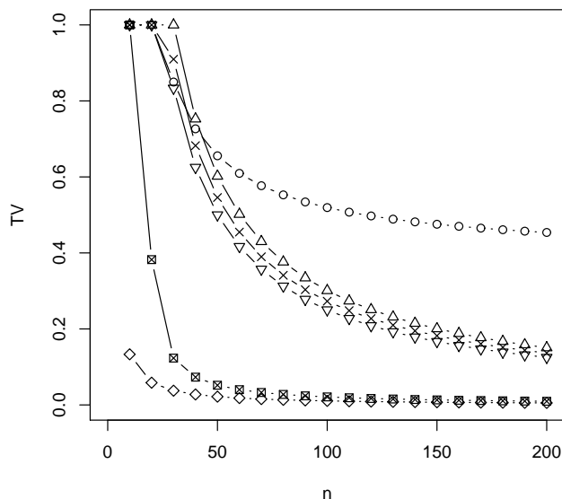
Figure 4: Bounds on the total variation distance d_{TV}(P_{S_n}, \text{CPo}(\lambda, Q)) for Q_i \sim \text{Geom}(\alpha_i) , where \alpha_i are uniformly spread between 0.15 and 0.25, n varies, and p is as in regime I, p = 5/n . Again, bounds based on J_{Q,1} are plotted as \circ ; those based on J_{Q,2} as \Delta ; Le Cam's bound in (6.1) as \nabla ; the Stein's method bound in (6.7) as \times , and Roos' bound from Theorem 2 of [33] as \boxtimes . The true total variation distances, computed numerically in each case, are plotted as \diamond .
