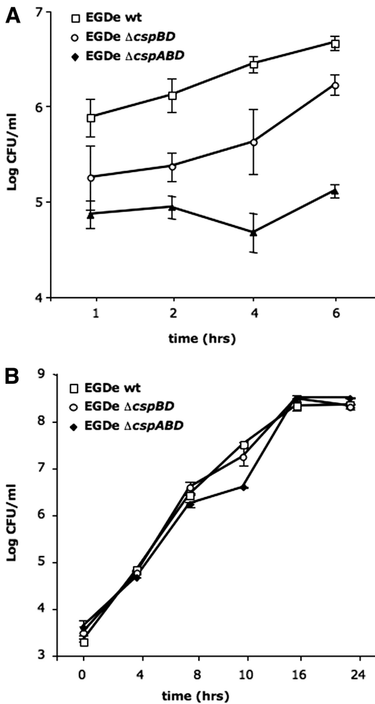
FIG. 4. Growth behavior of wild-type ( \square ), \Delta cspBD ( \circ ), and \Delta cspABD ( \blacktriangle ) strains in (A) infected J774.1 macrophages cultured at 37°C and (B) brain heart infusion culture in a shaking incubator held at 37°C. The three strains were analyzed as duplicates per experiment in three independent assays, and bars reflecting the mean and error ( \pm 1 SD) based on three independent analyses of each strain are presented.
