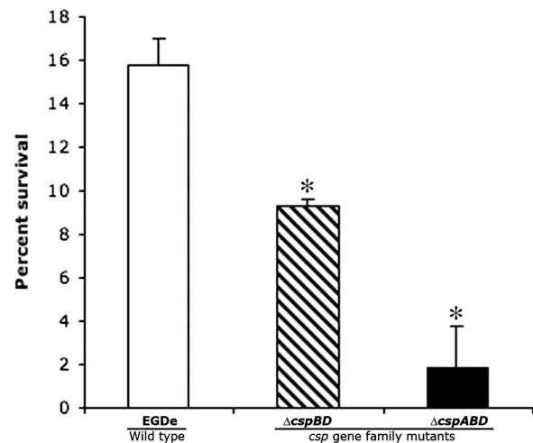
FIG. 5. Oxidative stress survival capacity of wild-type, \Delta cspBD , and \Delta cspABD strains. The percent survival (percentage of original inoculum surviving after 15 minutes in brain heart infusion plus 15 mM cumene hydroxyperoxide at 37°C) of the strains is displayed on the y-axis. The three strains were analyzed as duplicates in three independent assays, and bars reflecting the mean and error ( \pm 1 SD) based on three independent analyses of each strain are presented. The \Delta cspBD and \Delta cspABD strains displayed significantly ( p < 0.05 ; Wilcoxon/Kruskal-Wallis rank-sum test) lower survival of oxidative stress conditions compared with the wild-type strains as indicated by an asterisk above each bar.
