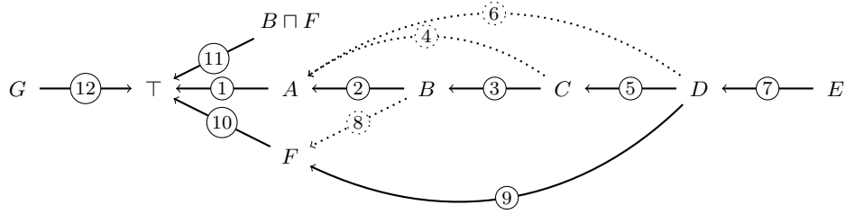
Fig. 1. Example TBox. Nodes correspond to concepts and arcs correspond to subclass inclusions. Dotted arcs represent disjoints. The axioms are numbered for referring to them in the text. Below, the root justifications for the non-purely derived unsatisfiable concepts are shown.
