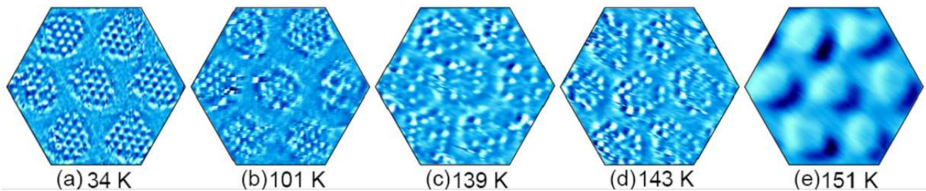
FIG. 3: Behavior of nano-ice clusters in the temperature range between 34 K and 151 K as recorded by variable temperature scanning tunneling microscopy (VT-STM). The 5 hexagonal frames with a side length of 4.2 nm show the constant current feed-back signal, after drift correction. (a) Nano-ice clusters at 34 K. V_t = -0.05 V, I_t = 100 pA. (b) At 101 K water molecules at the rims of the nano-ice cluster become mobile, the core remains frozen. V_t = -0.05 V, and I_t = 100 pA. (c) Low coordinated water induced protrusions at the cluster boundary are observed at 139 K, the core features weaken. V_t = -0.01 V, and I_t = 50 pA. (d) as (c), the rims show higher contrast than the core molecules which still show crystallinity at 143 K. V_t = -0.01 V, and I_t = 50 pA. (e) Empty nanomesh after water desorbed from the surface. V_t = -0.05 V, and I_t = 40 pA.
