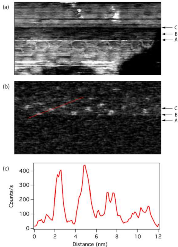
FIG. 4: Room temperature scanning tunneling microscopy and photon emission scanning tunneling microscopy from h -BN nanomesh with a gold coated tungsten tip. ( 30 \times 15 nm, I_t = 2.6 nA, V_t = -2.5 V, scan time 110 s with 128 horizontal scanning lines from bottom to top). The labels A, B, C indicate tip changes (for details see text). a) Topography, note the 3 nm periodicity of h -BN nanomesh, and the tip changes A, B . b) Light map, i.e. simultaneously to a) recorded photon current. For a certain line series the luminescence is particularly high, and the periodicity of the h -BN nanomesh lights up. c) Cut across the light map, along the red line in b). The polychromatic light current is given in photons/s.
