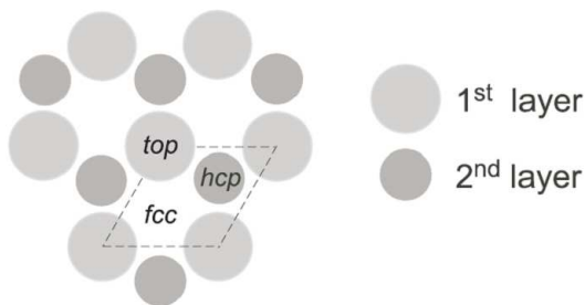
FIG. 1: Scheme for the classification of the adsorption sites on a hexagonal closed packed surface: top , fcc , and hcp . The dashed line shows the (1 \times 1) unit cell. After Ref. [14]
