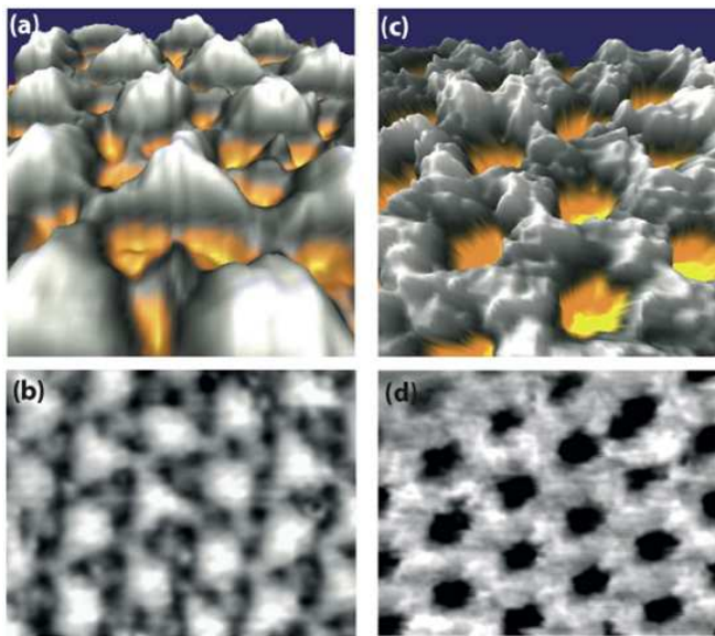
FIG. 2: Scanning tunneling microscopy data of sp^2 single layers on Rh(111). a) Relief view of g /Rh(111). Note the hills and the valleys, and the small extra hills at the (hcp, fcc) sites. b) corresponding STM picture ( I_t = 0.8 nA, U_t = -0.8 V, 11 \times 14 nm 2 ). c) Relief view of h -BN/Rh(111) nanomesh. The elevated regions form the so called wires of the nanomesh. d) corresponding STM picture ( I_t = 1 nA, U_t = 1 V, 11 \times 14 nm 2 ).
