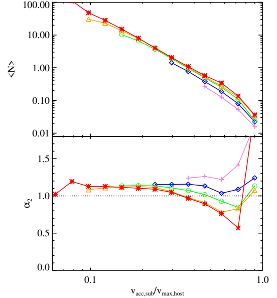
FIG. 3.— Top Panel : The trend of \langle N \rangle for the v_{acc} distribution function for hosts of varying masses. This is equivalent to the subhalo mass function. Magenta pluses, blue diamonds, green circles, and red triangles represent hosts with v_{max} = 200, 300, 600, and 1000 \text{ km s}^{-1} , respectively. Bottom Panel : The trend of the scatter in the distribution of the number of subhalos above a mass threshold. The dashed line represents \alpha_2 = 1 , where the negative binomial distribution reduces to Poisson.
