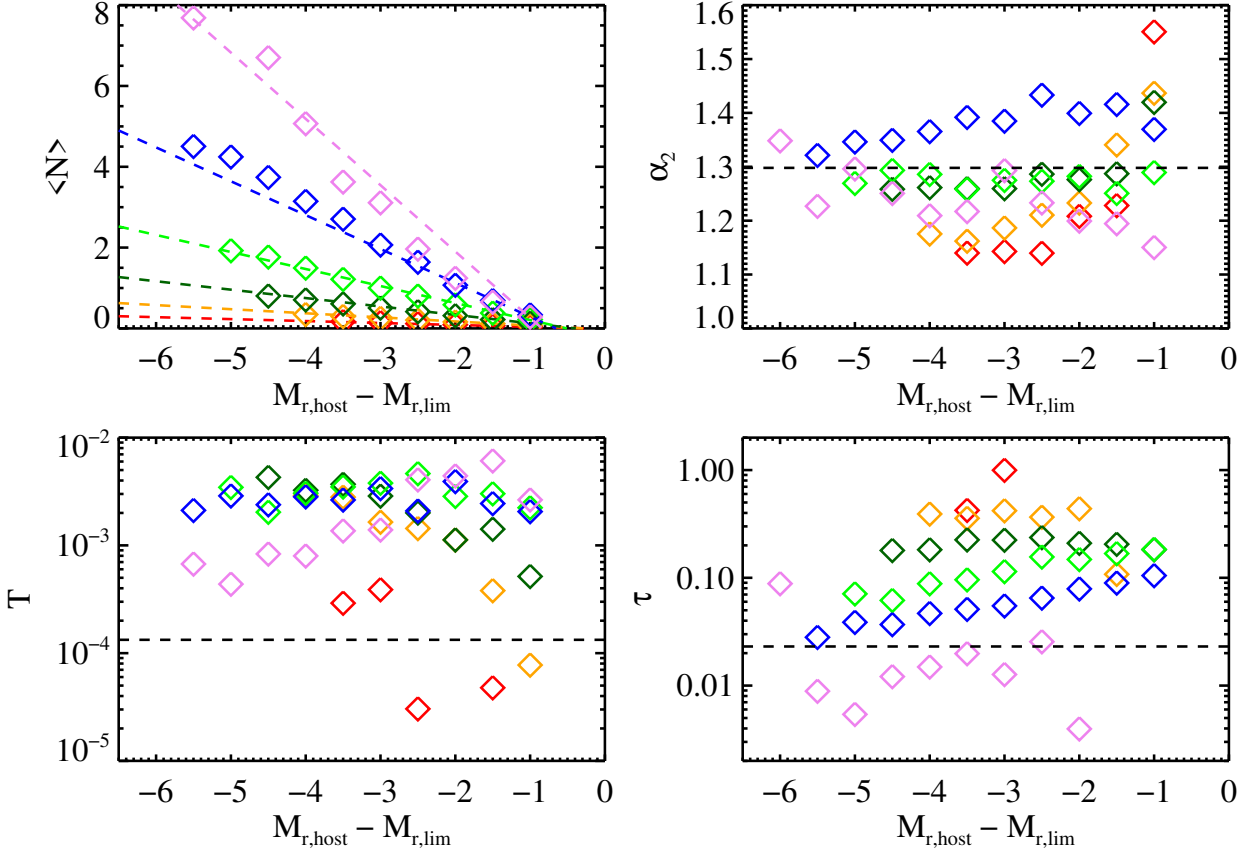
FIG. 13.— The fit parameters specifying the P(N) distribution (equation 6) as a function limiting satellite magnitude, represented as a magnitude difference (luminosity ratio). Different colored points represent different host populations: violet, blue, green, dark green, orange, and red points are hosts with M_r = -19.8, -20.3, -20.8, -21.3, -21.8, and -22.3 . Dashed lines represent our fits to these distributions, as given in Equation 7.
